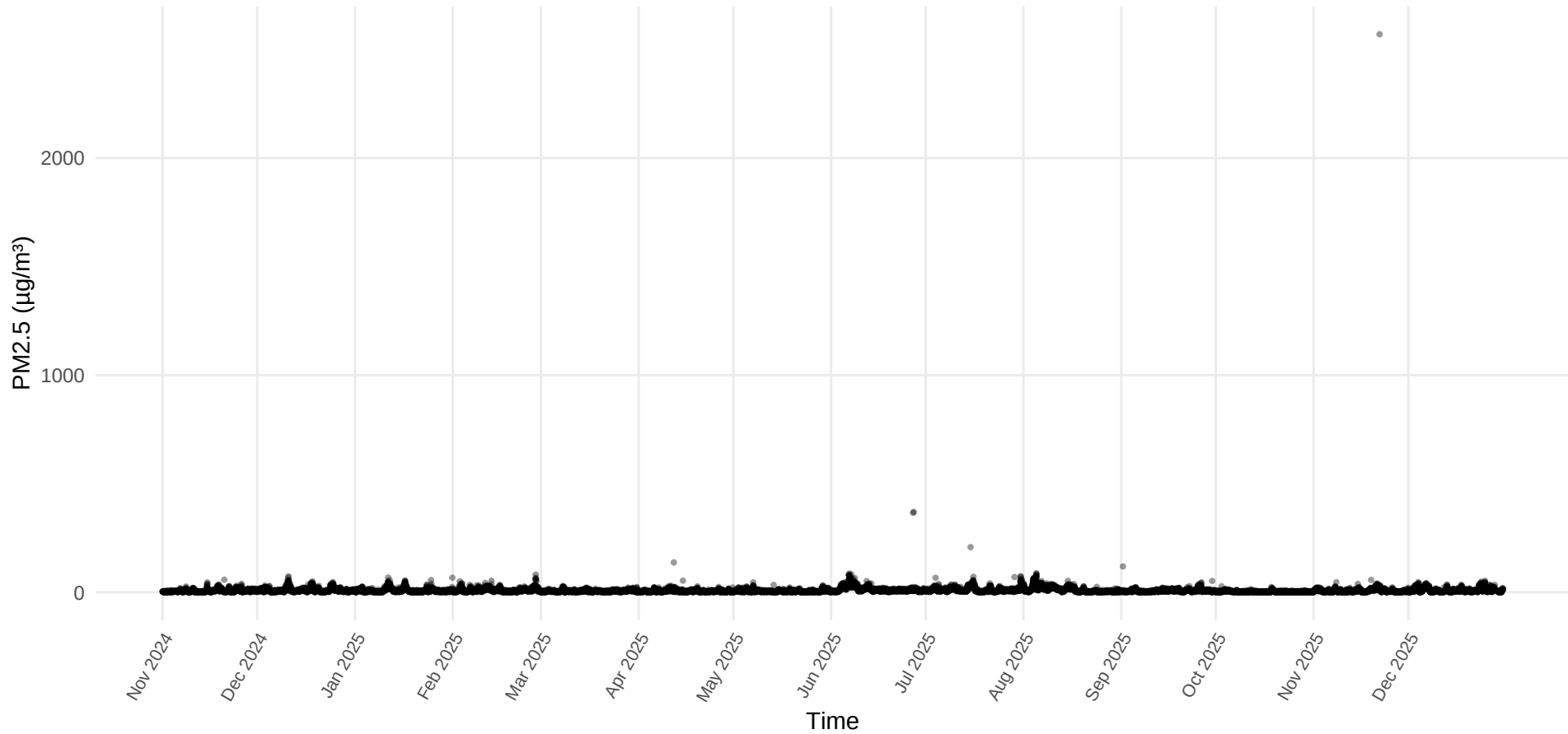
PM2.5 Time Series – Site 3.1 (Device 3 – Nottingham Water )
