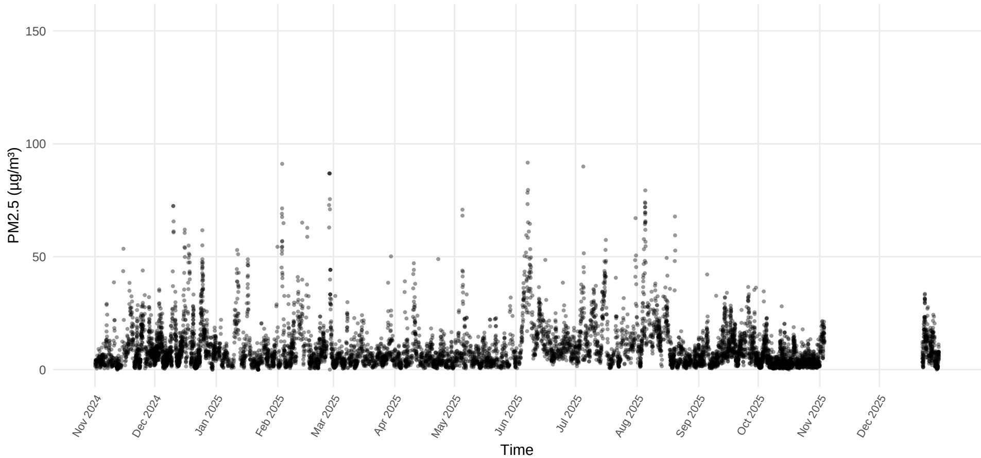
PM2.5 Time Series – Device 8 – East 56th Street and Ferro Avenue
