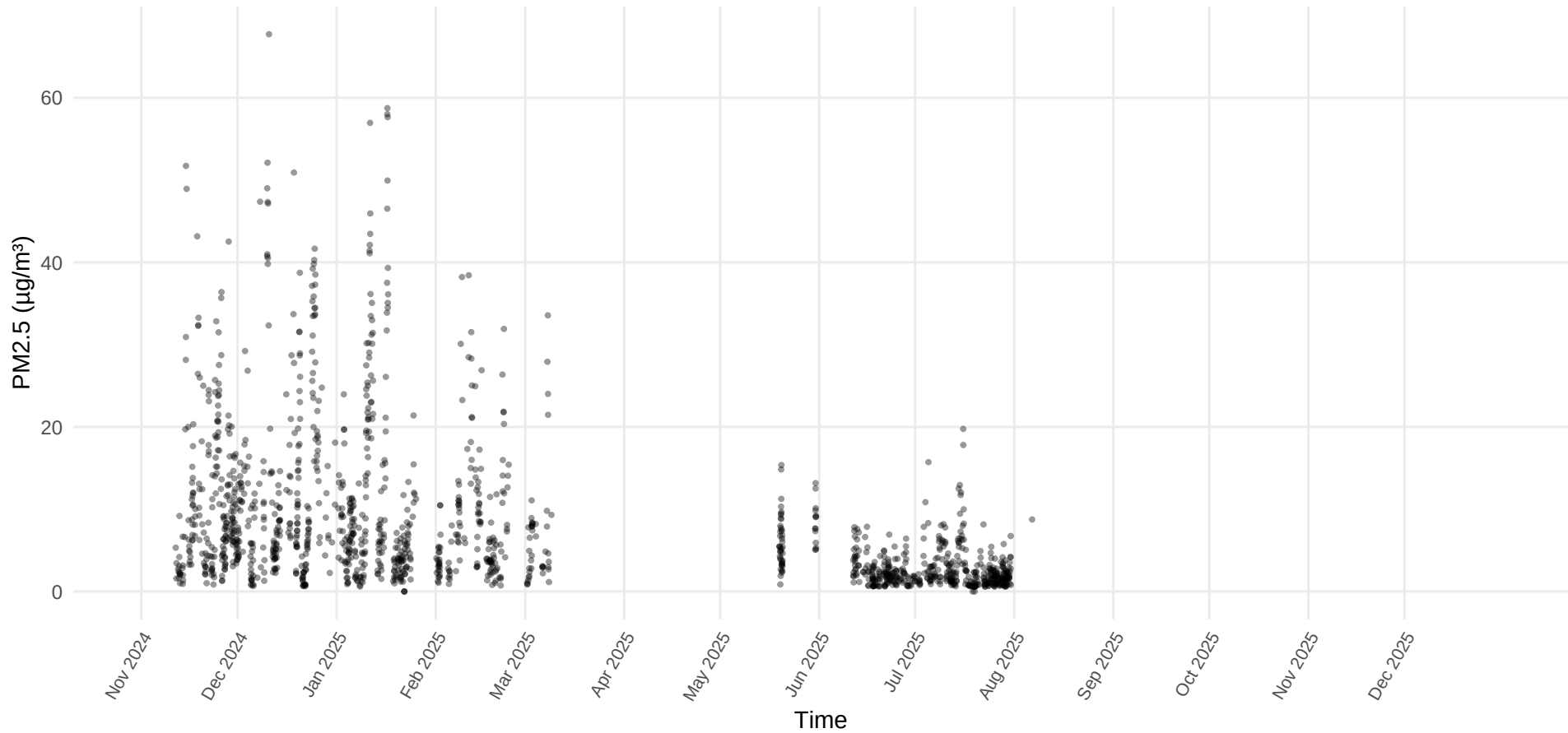
PM2.5 Time Series – Site 1.1 (Device 1 – Fleet Ave. and East 71st St. )
