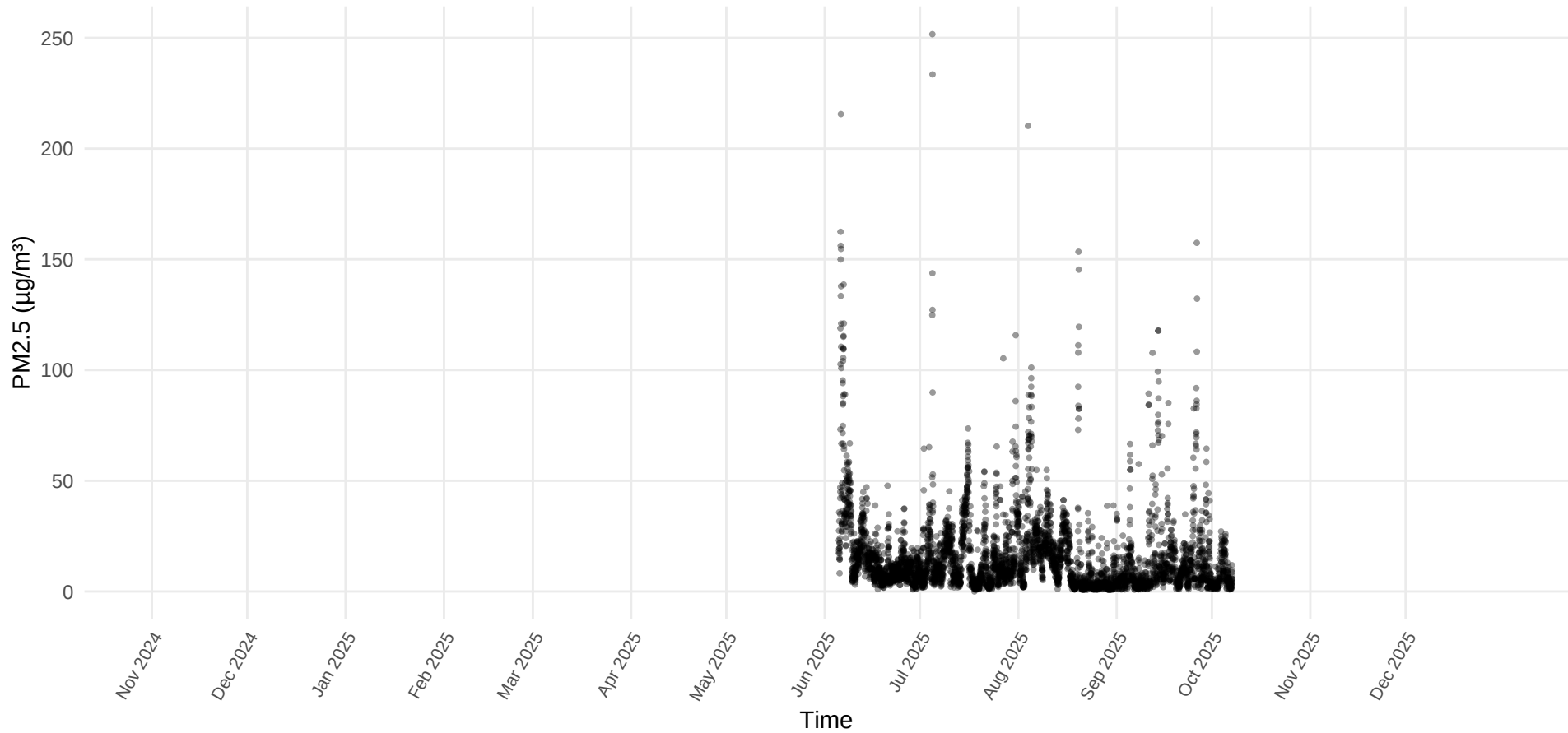
PM2.5 Time Series – Site 34.1 (Device 34 – Clark Recreation Center )
