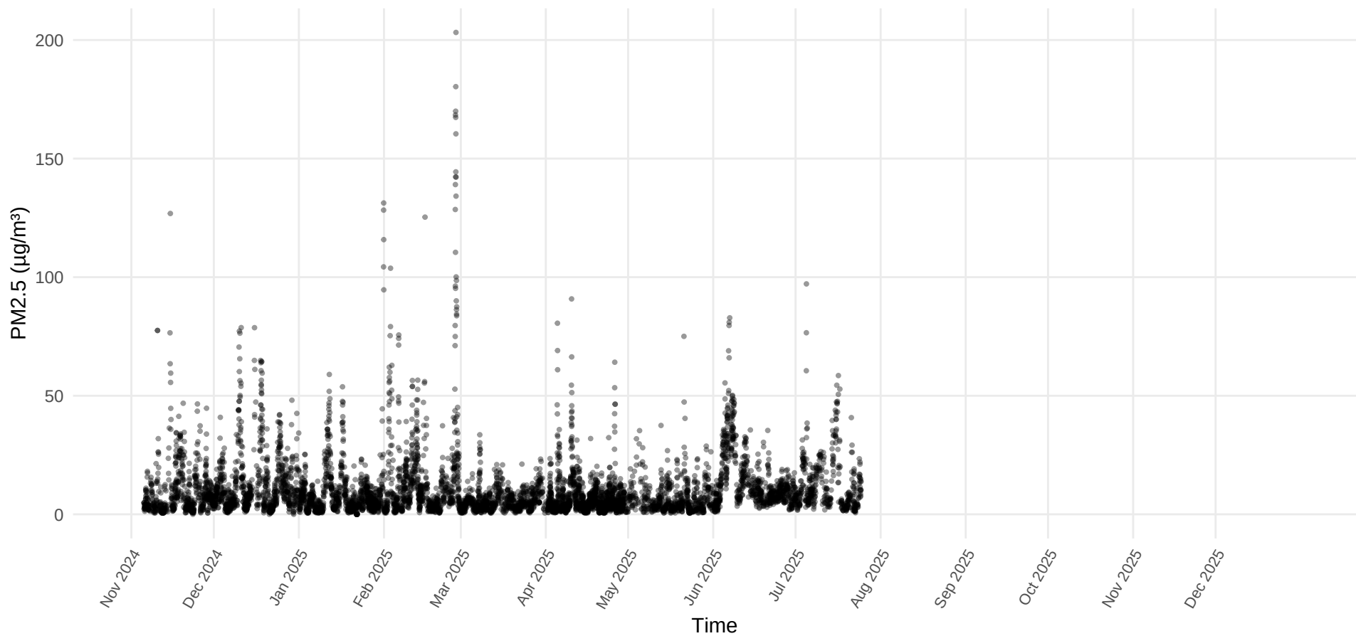
PM2.5 Time Series – Site 7.1 (Device 7 – St. Theodosius Monitoring Site Collocated Sensor )
