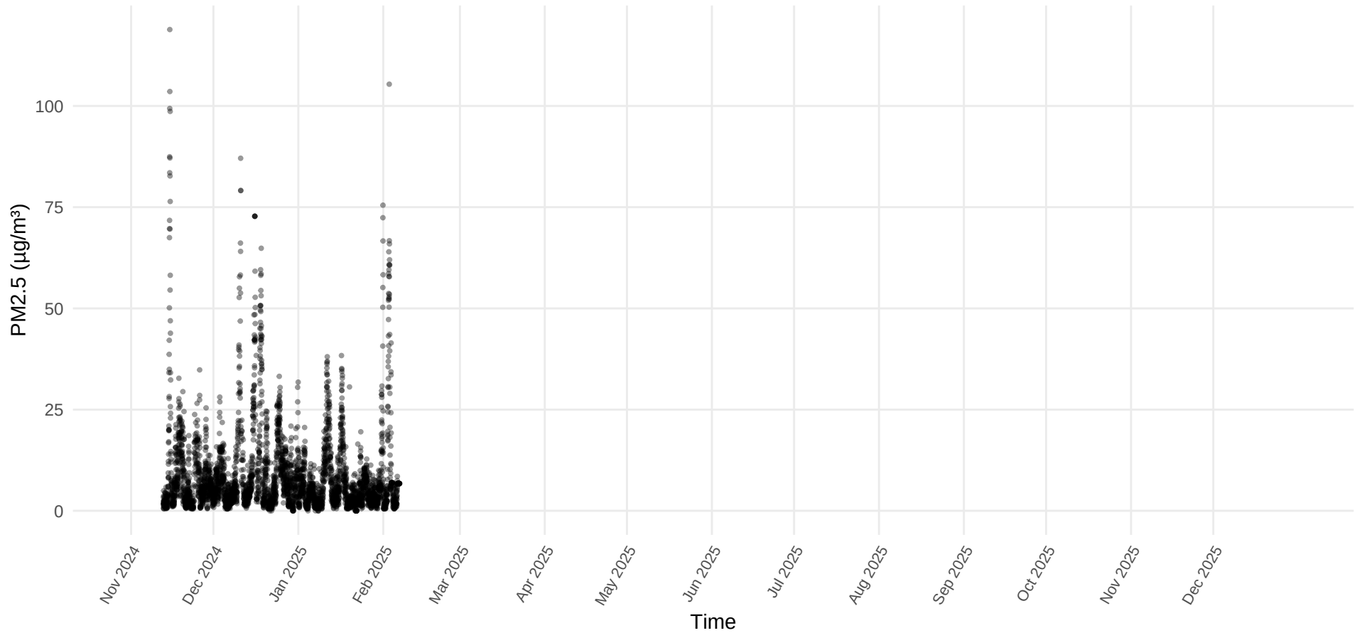
PM2.5 Time Series – Site 9.1 (Device 9 – GT Craig EPA Collocated Sensor )
