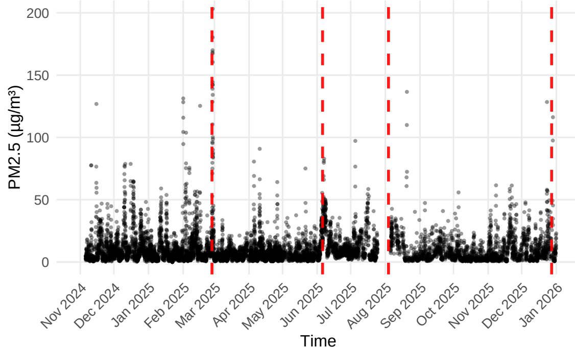
PM2.5 Time Series – Site 3.1
