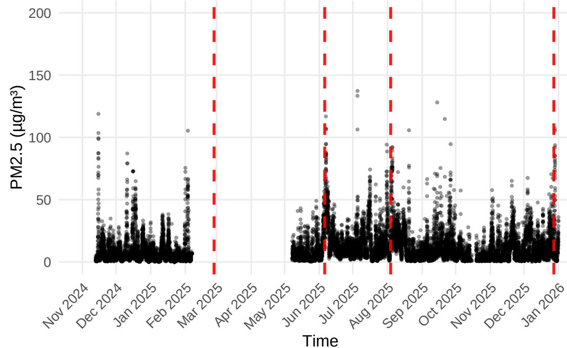
PM2.5 Time Series – Site 18.1_26.1
