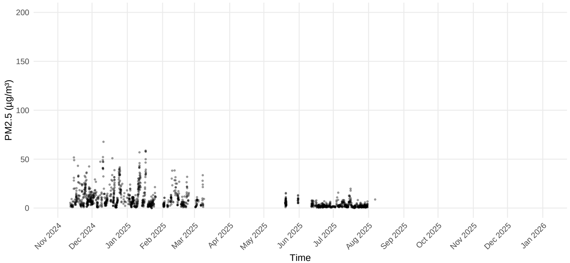
PM2.5 Time Series – Site 1.1
