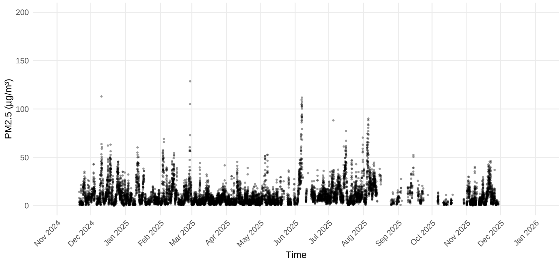
PM2.5 Time Series – Site 12.1_5.2
