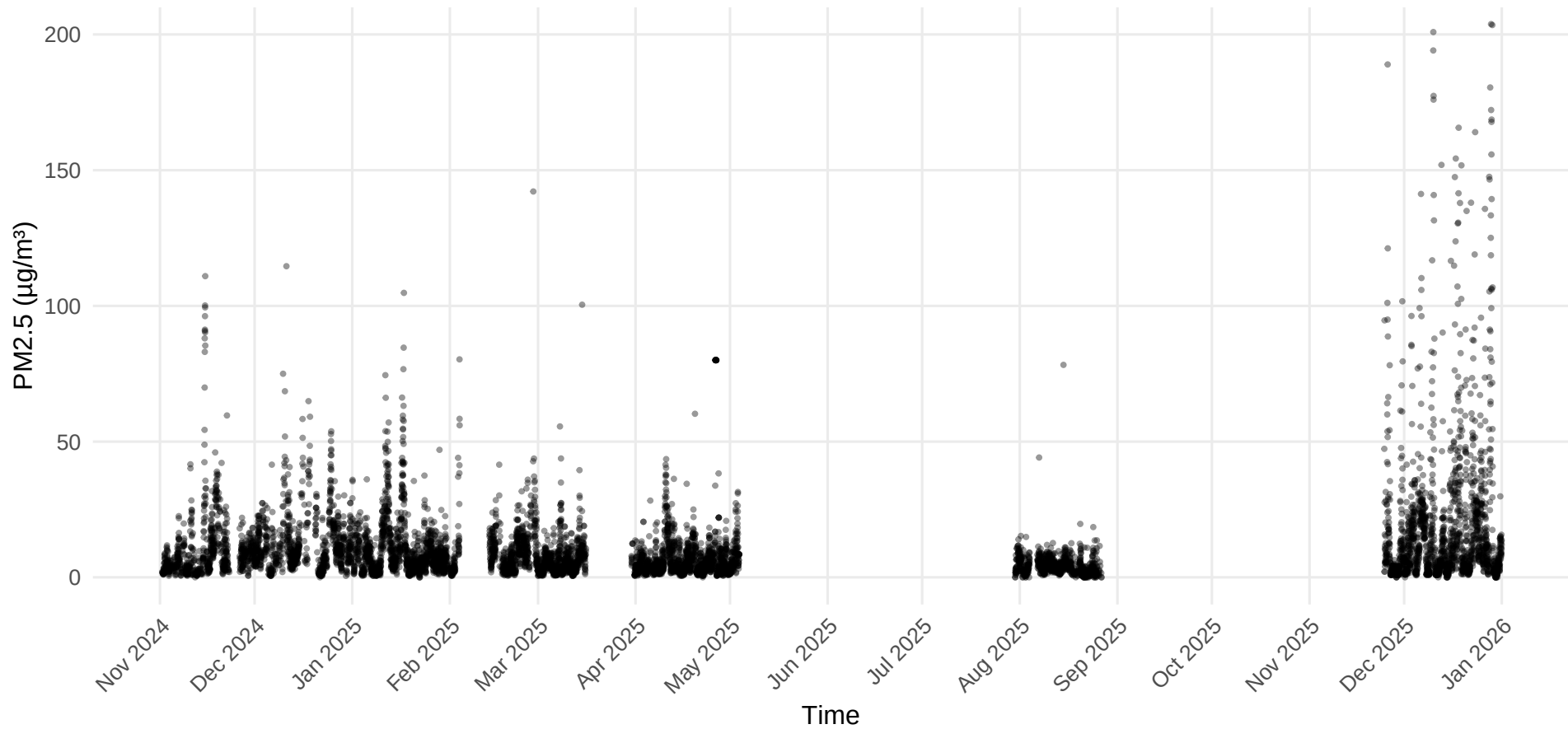
PM2.5 Time Series – Site 13.1_33.2
