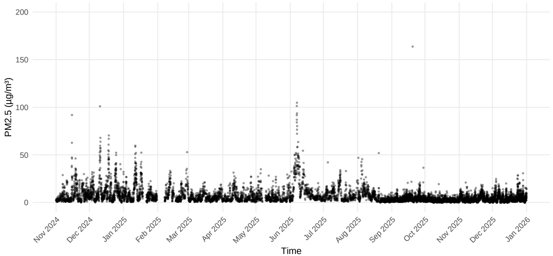
PM2.5 Time Series – Site 15.1
