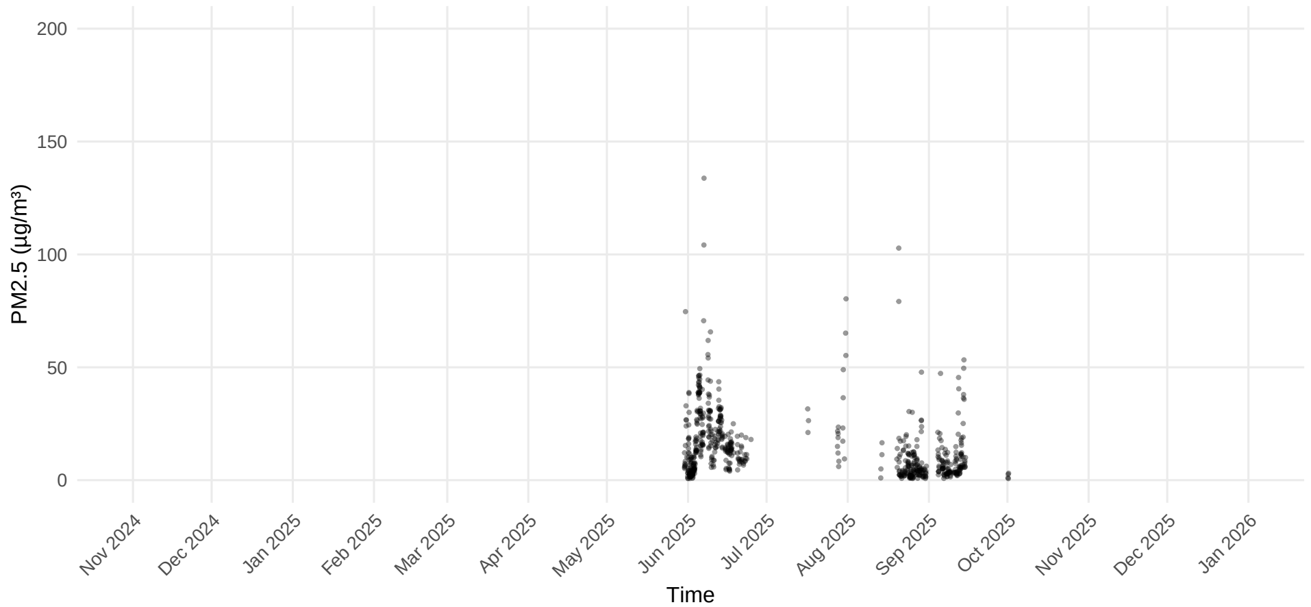
PM2.5 Time Series – Site 19.2
