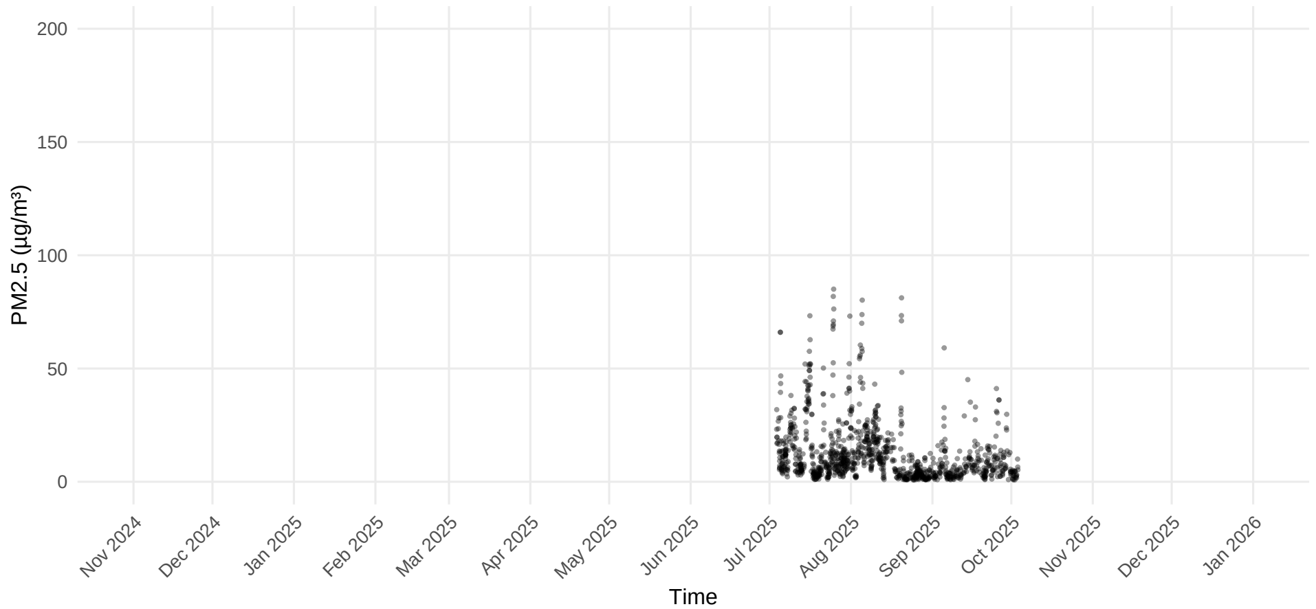
PM2.5 Time Series – Site 33.1
