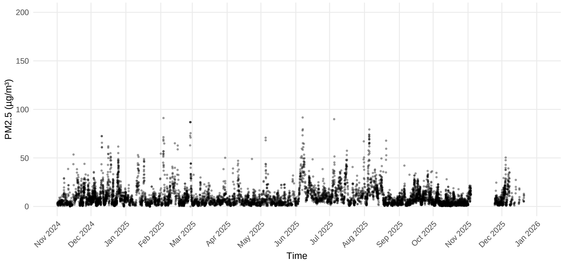
PM2.5 Time Series – Site 8.1_34.2
