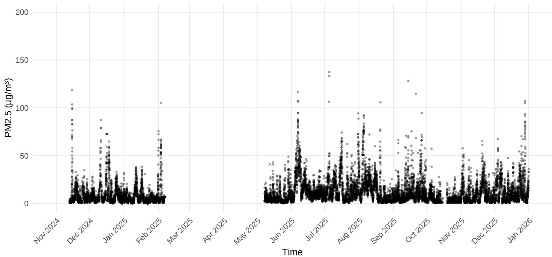
PM2.5 Time Series – Site 9.1_17.2
