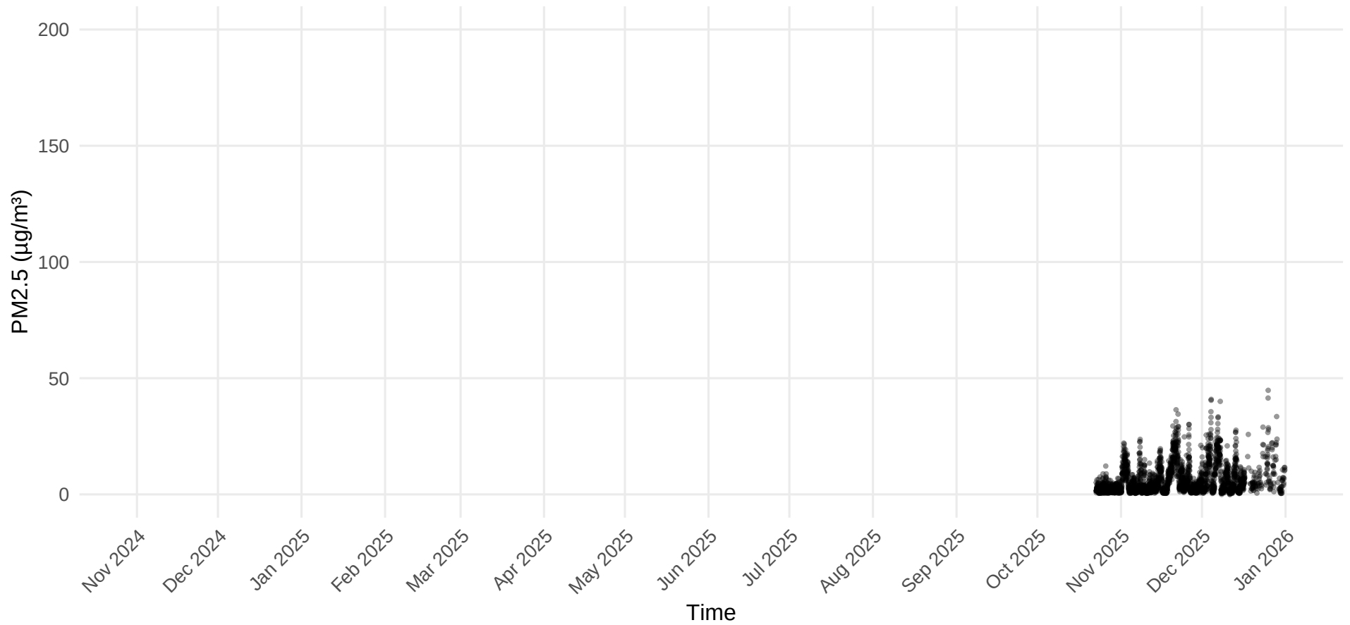
PM2.5 Time Series – Site 9.2
