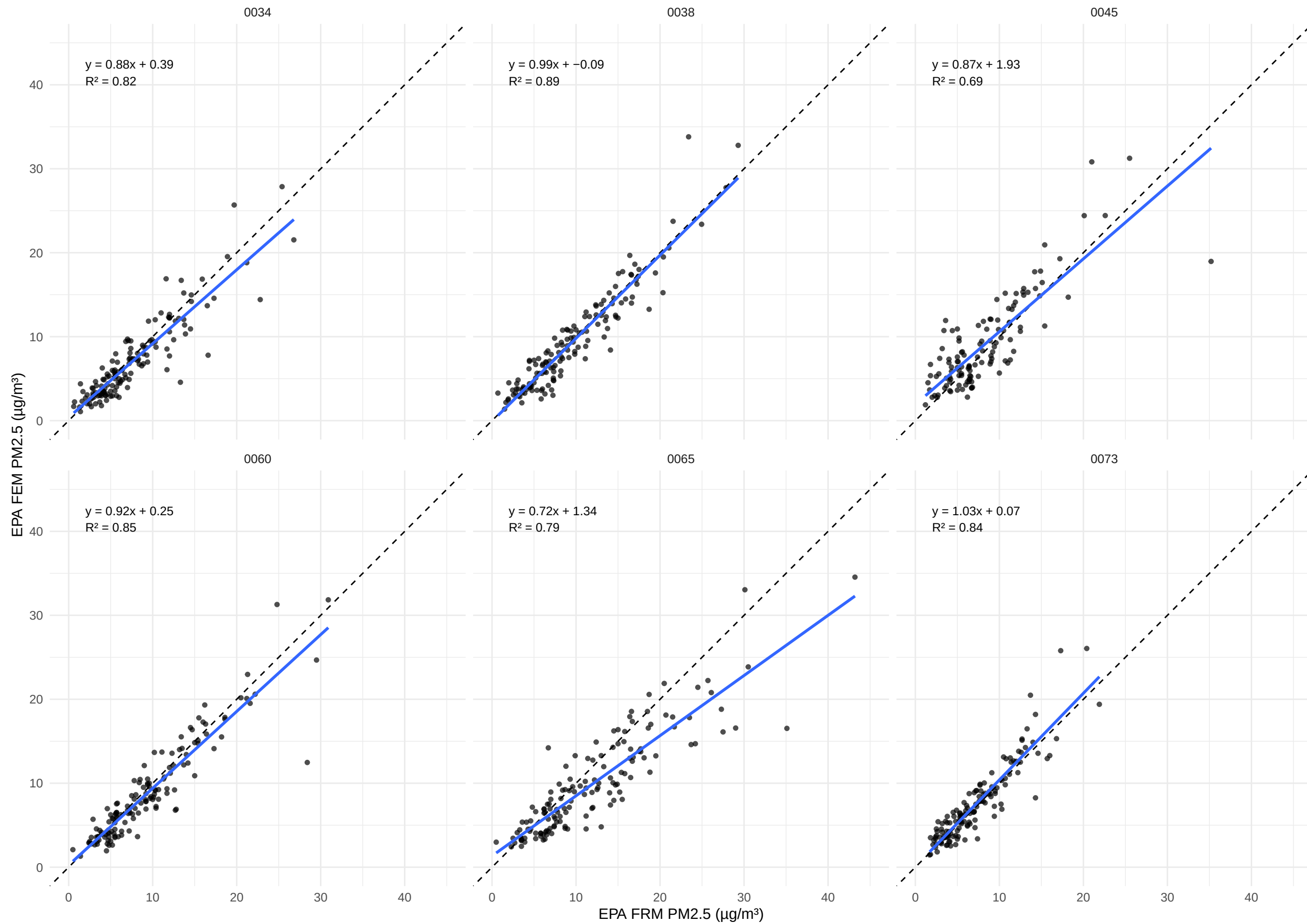
Figure C. EPA FEM vs FRM at Same Site FEM daily averages screened using at least 18 hourly observations
