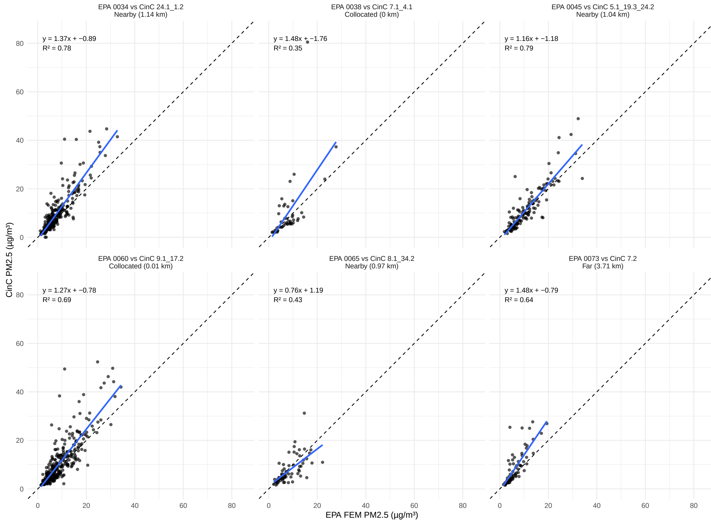
Figure E. CinC vs EPA FEM at Nearest Site
