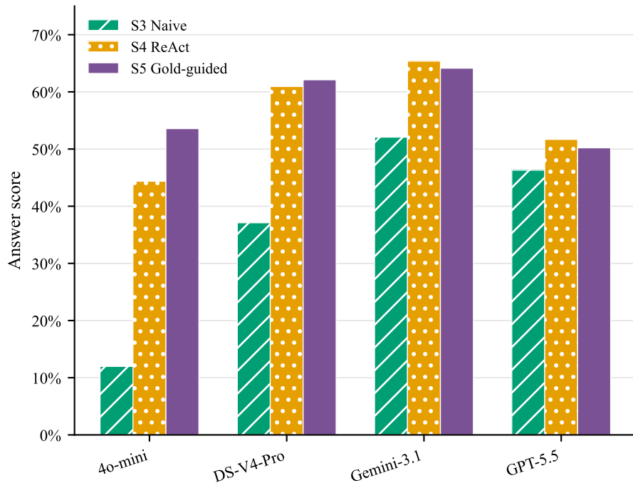
(b) Gold-surface intervention
