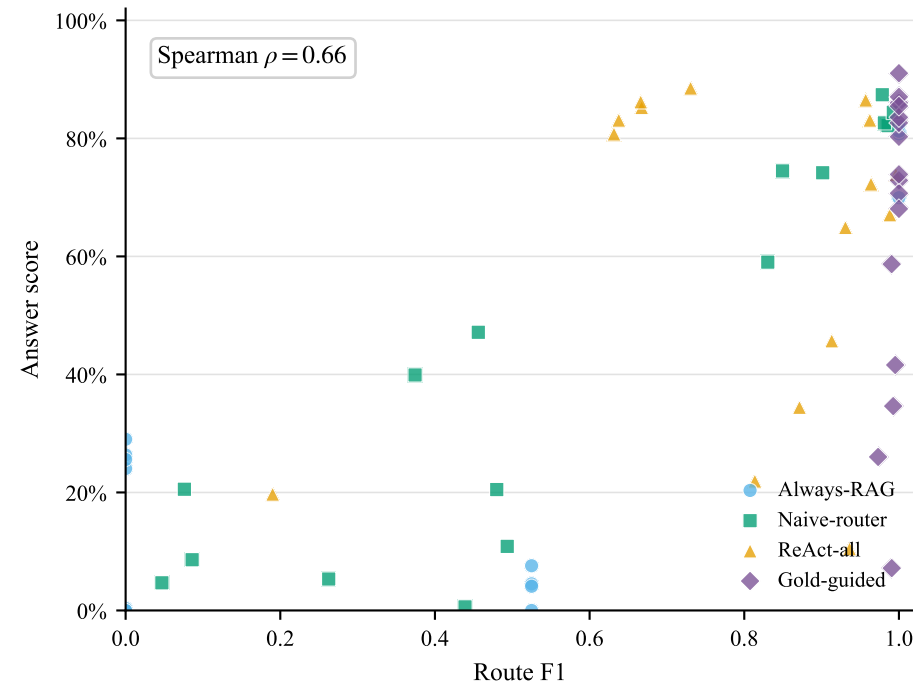
(a) Routing and answering
