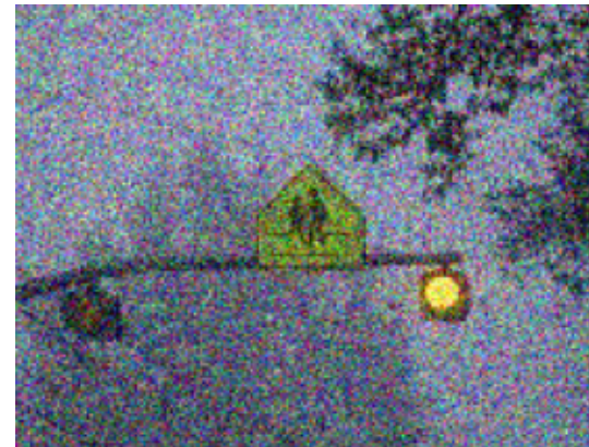
Severity 3
