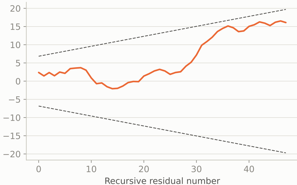
CUSUM (5% bands)
