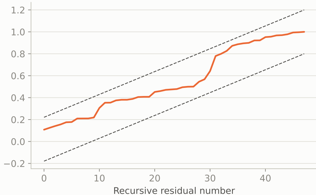
CUSUM of squares (5% bands)
