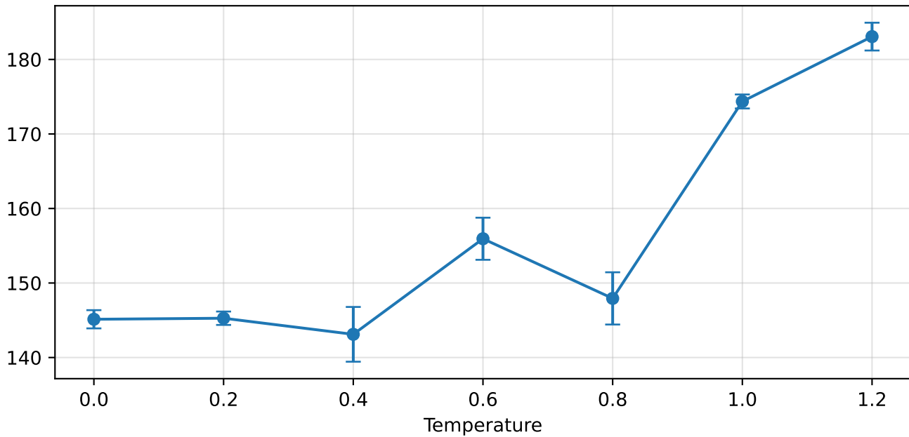
Mean output tokens
