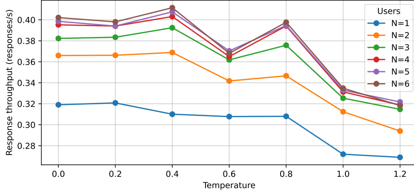
Fig. 8. Response throughput versus temperature for each number of users.
