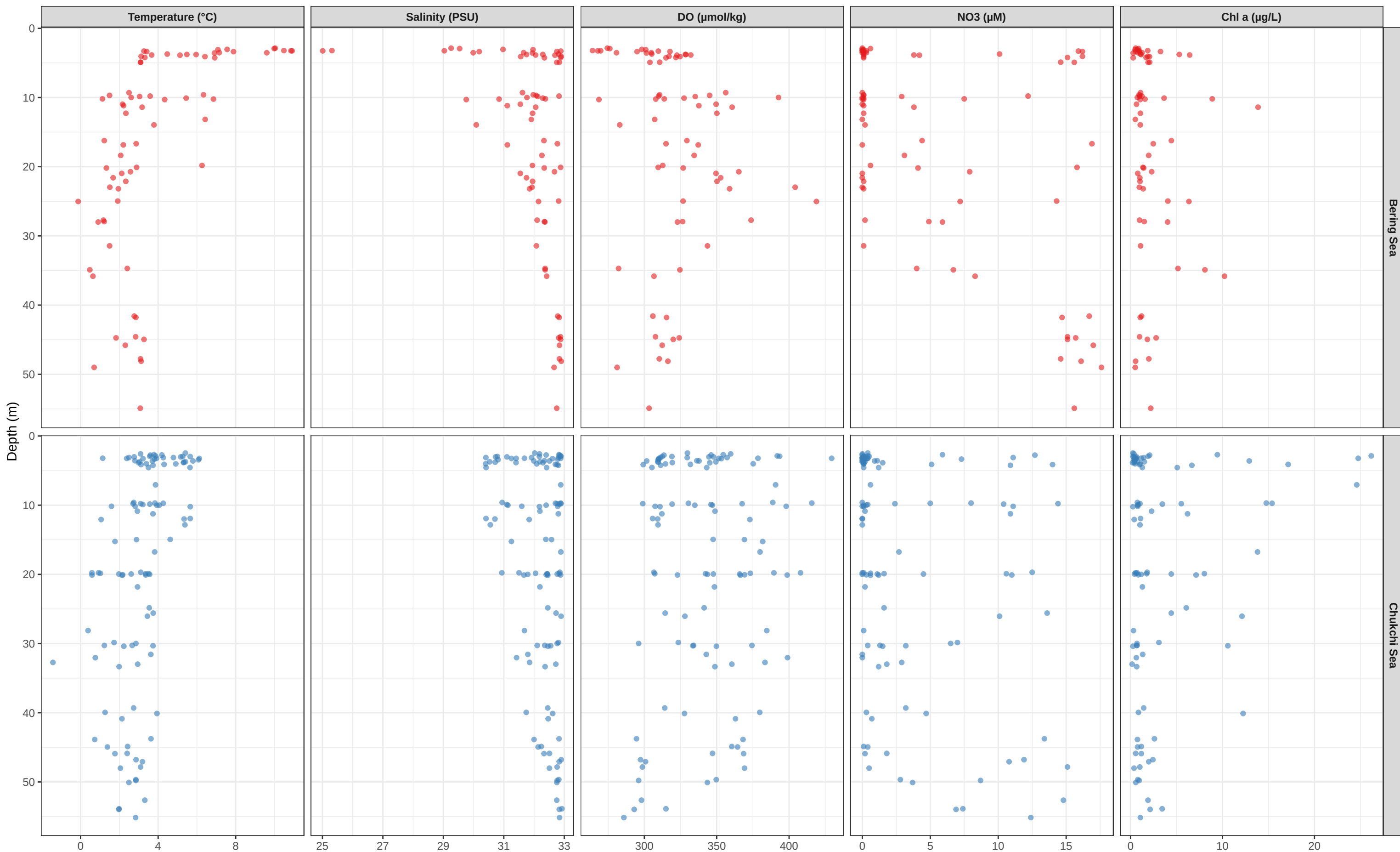
Vertical profiles by sea (rows) × variable (cols)
