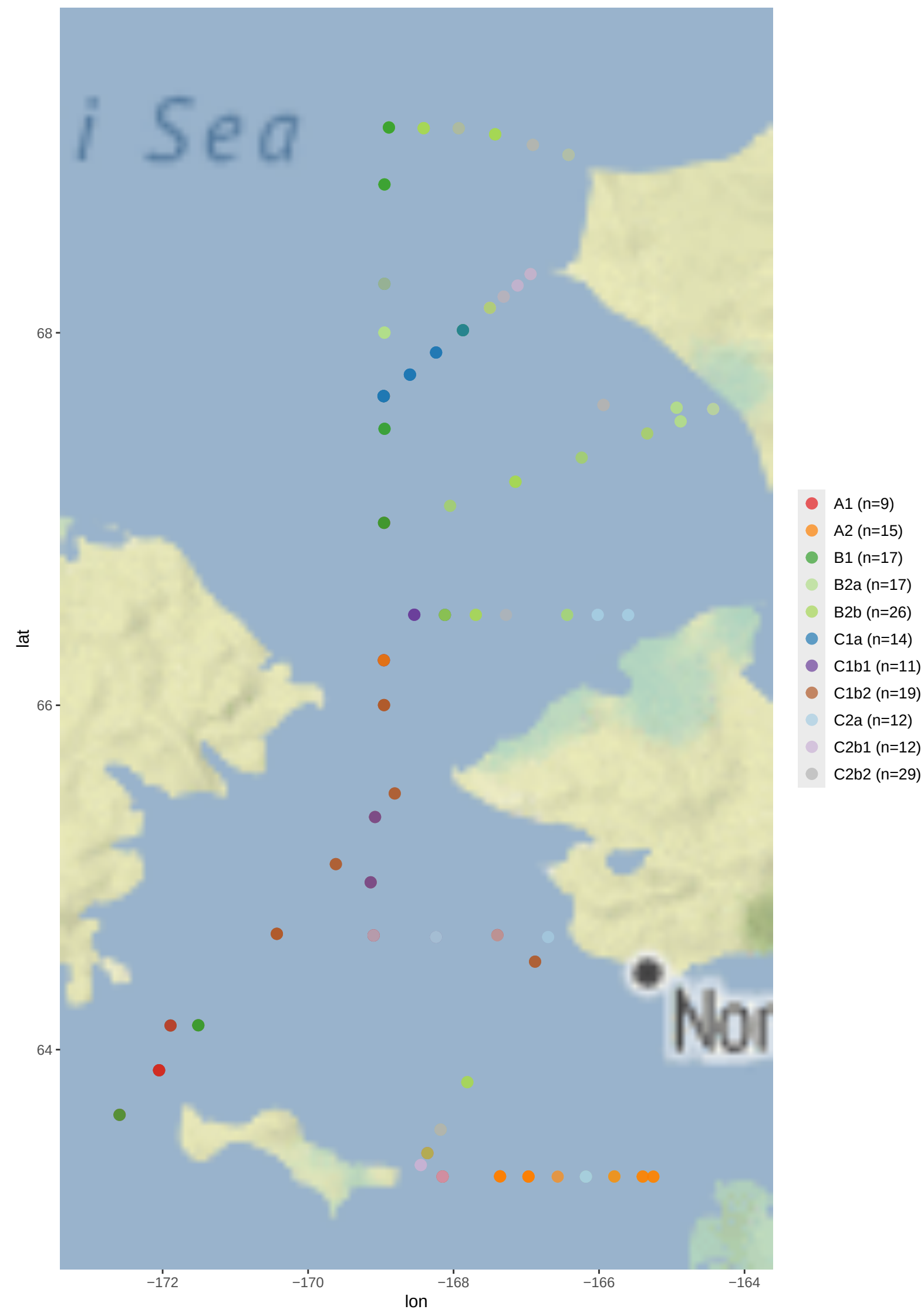
ASGARD 2017 Survey – 11 clusters
