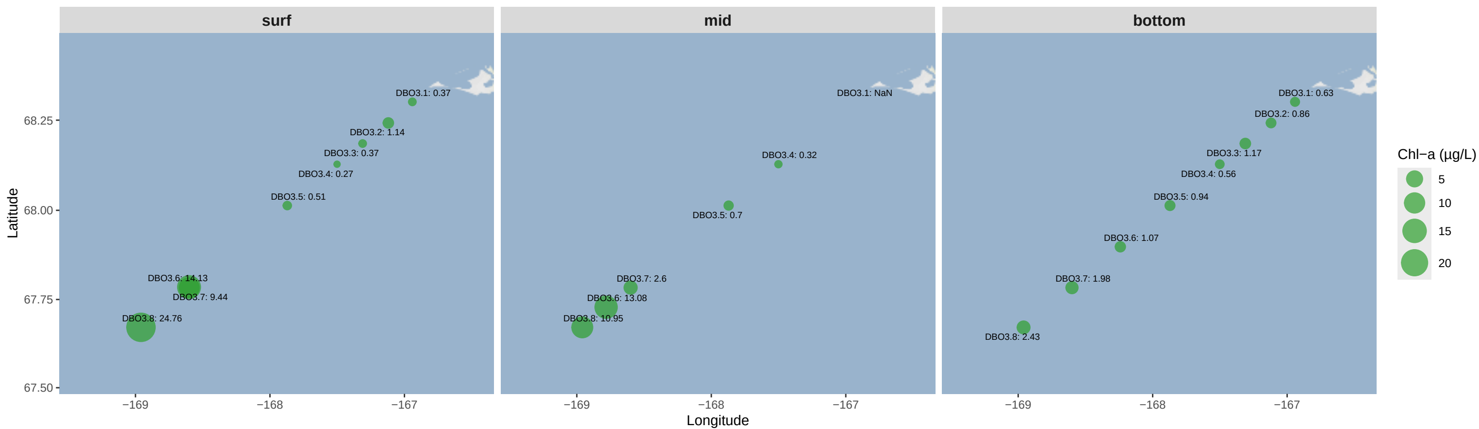
DBO3 Chl-a by depth type
