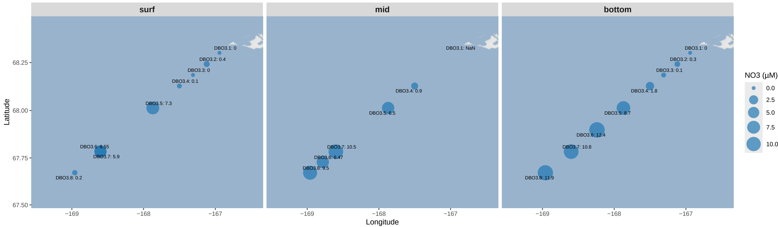
DBO3 NO3 by depth type
