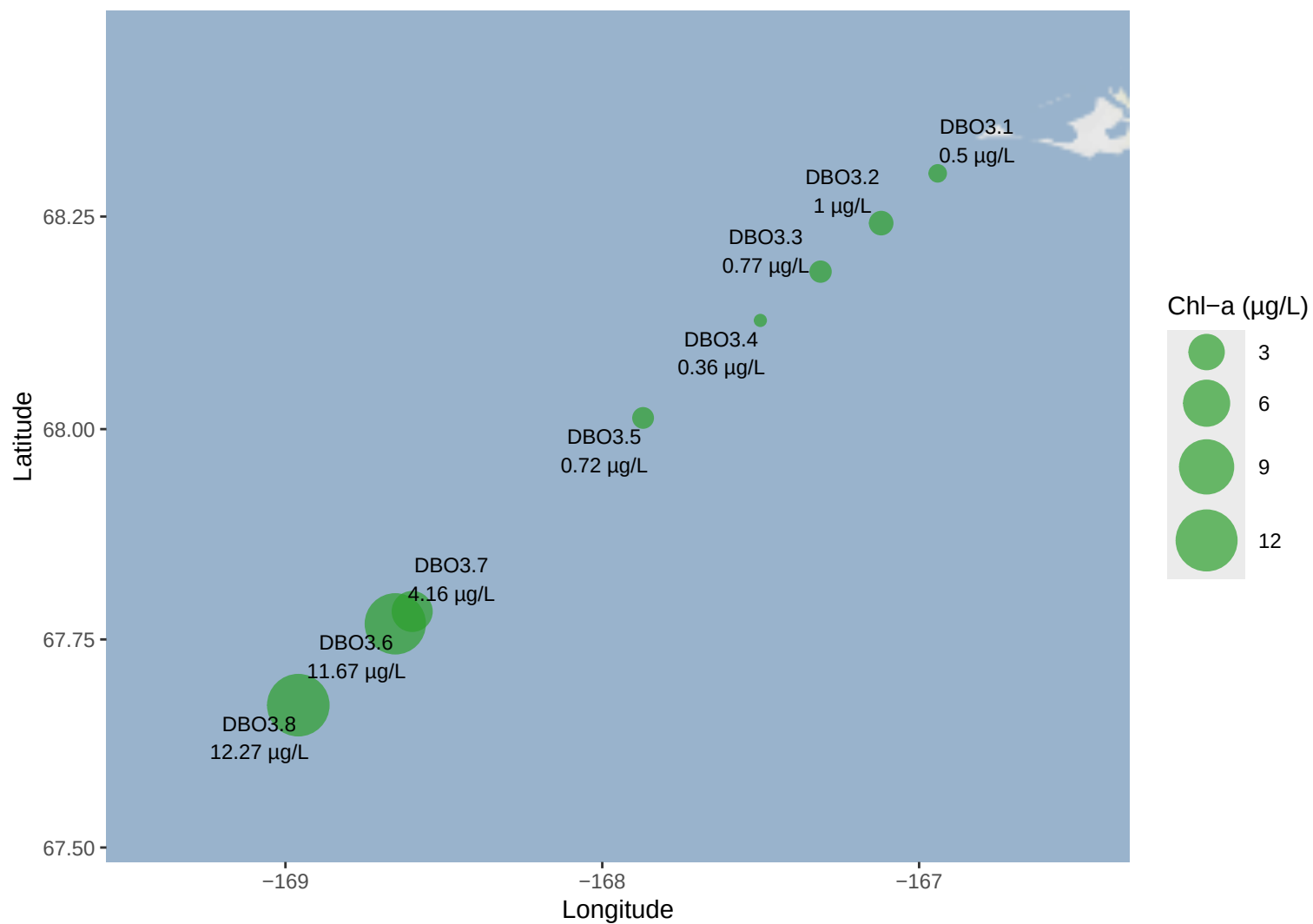
DBO3 station mean Chl-a (depth-averaged)
