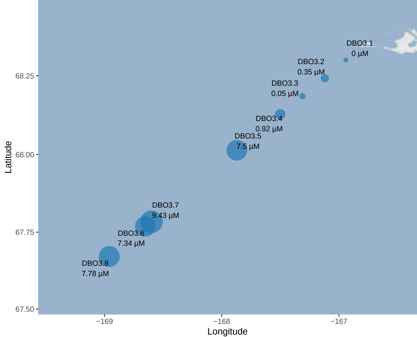
DBO3 station mean NO3 (depth-averaged)
