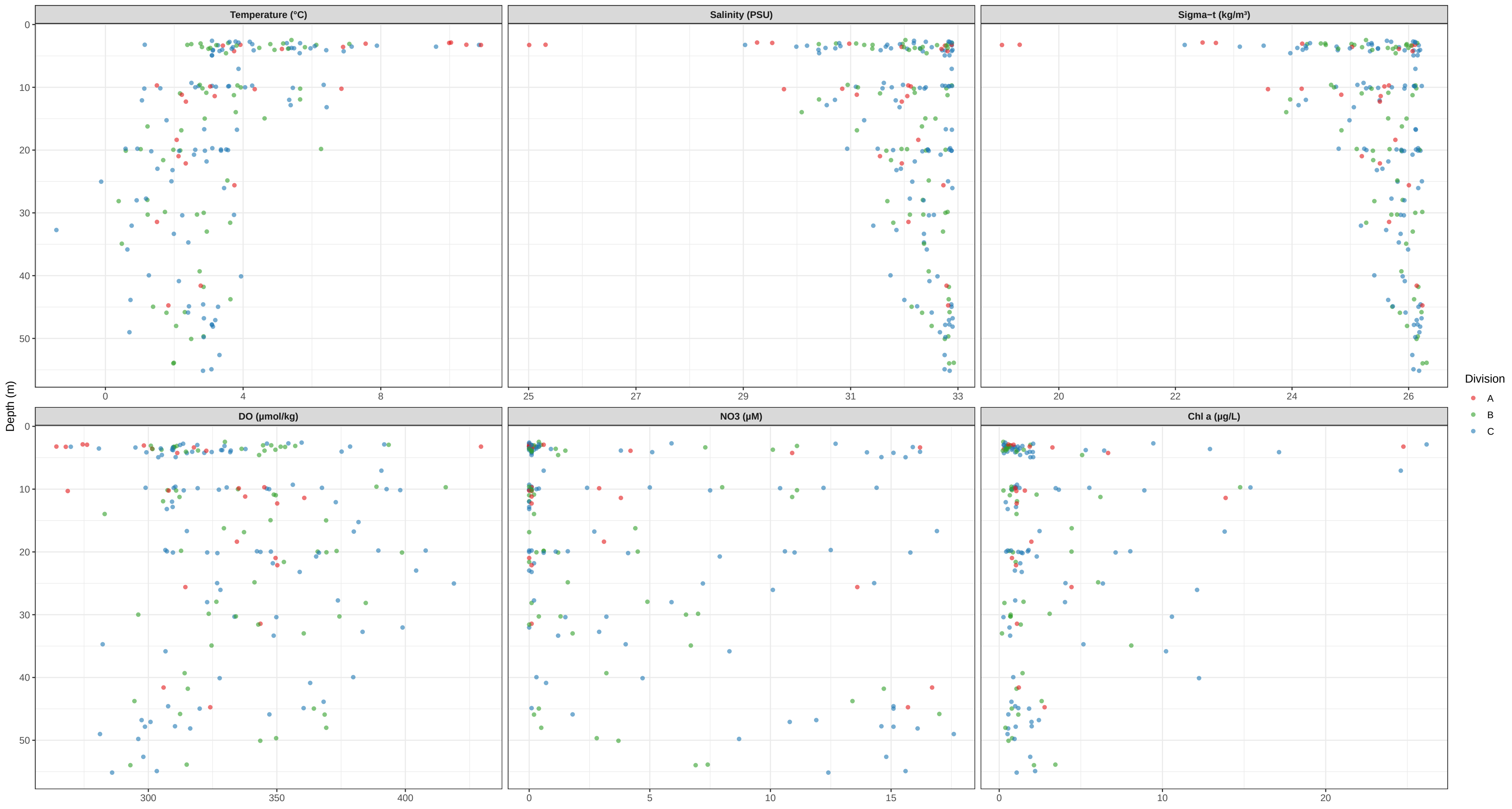
Vertical profiles by Division (A/B/C)
