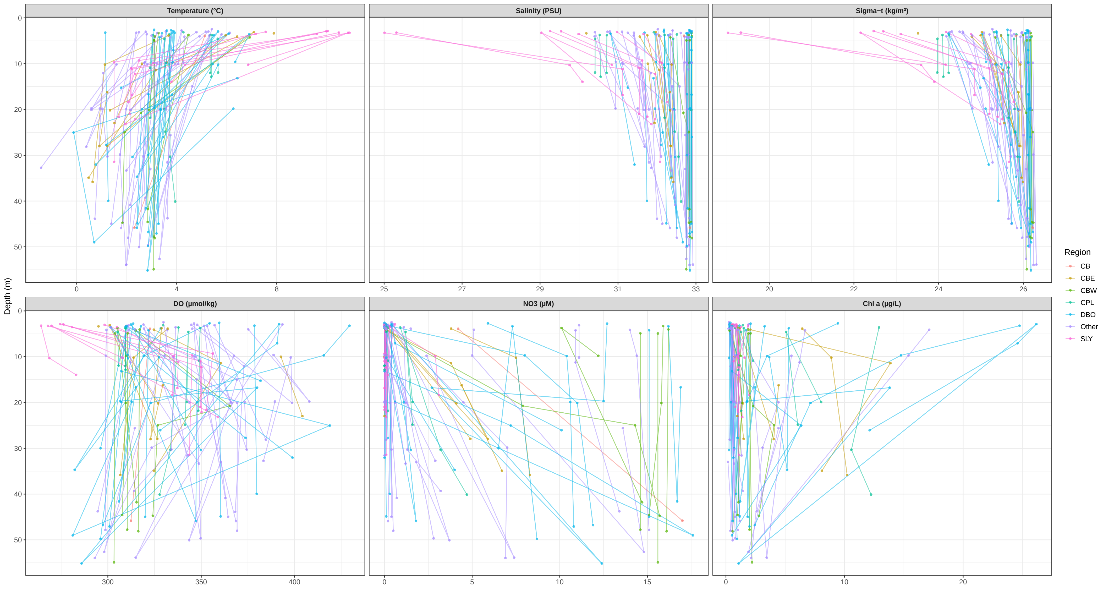
Per-station vertical profiles by transect region
