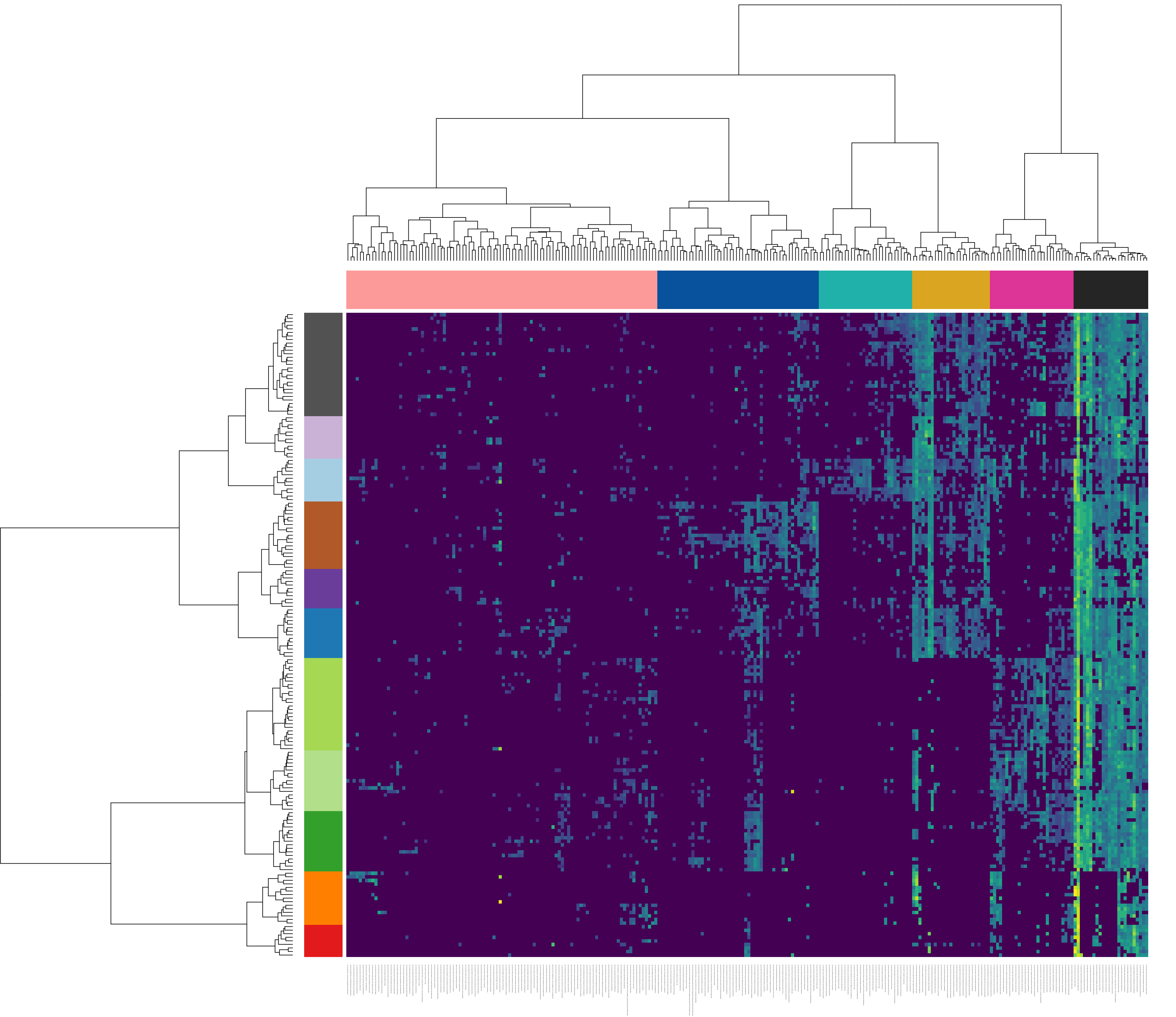
ASGARD Survey 16S – 11 clusters (ASV names)
