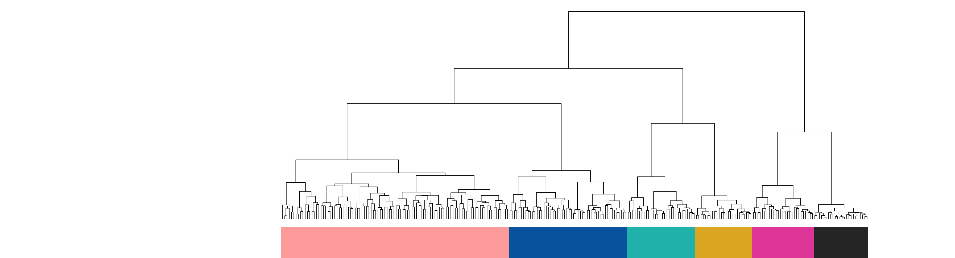
ASGARD Survey 16S – 11 row clusters, 6 col clusters
