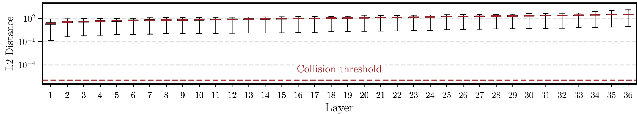
gpt2-large
