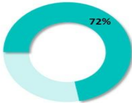
Quality Score
