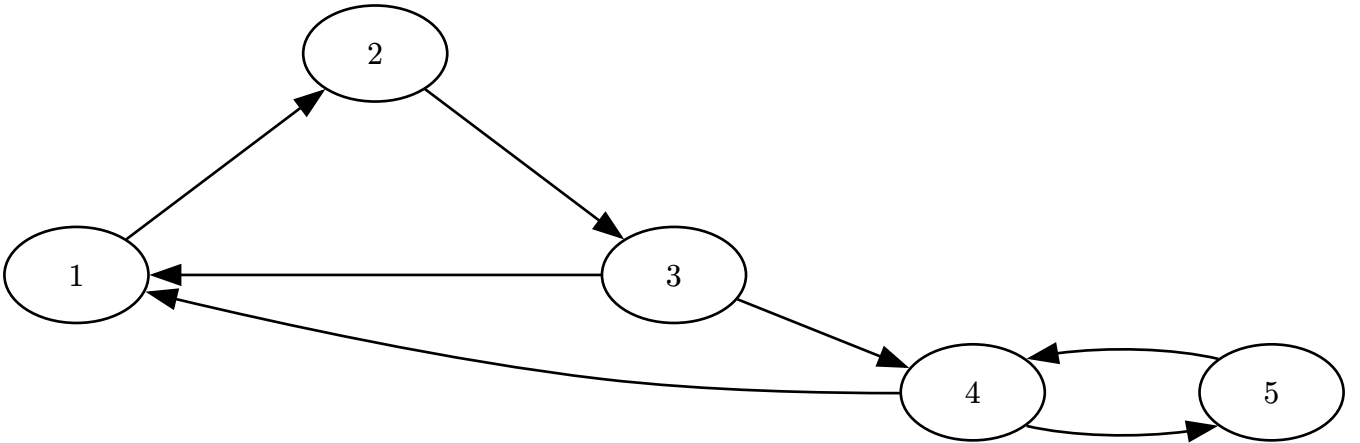
Figure 2: An example graph G.
