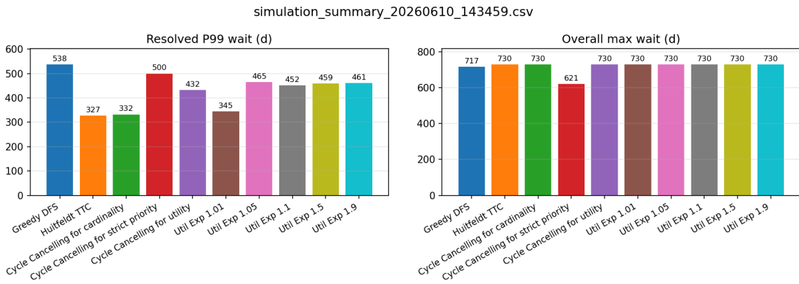
Figure 12: 99th percentile wait of resolved patients and overall maximum wait under each algorithm in the small simulation with exponential variants, over 730 days. The maximum is taken over all patients, including those still waiting when the simulation ended.
