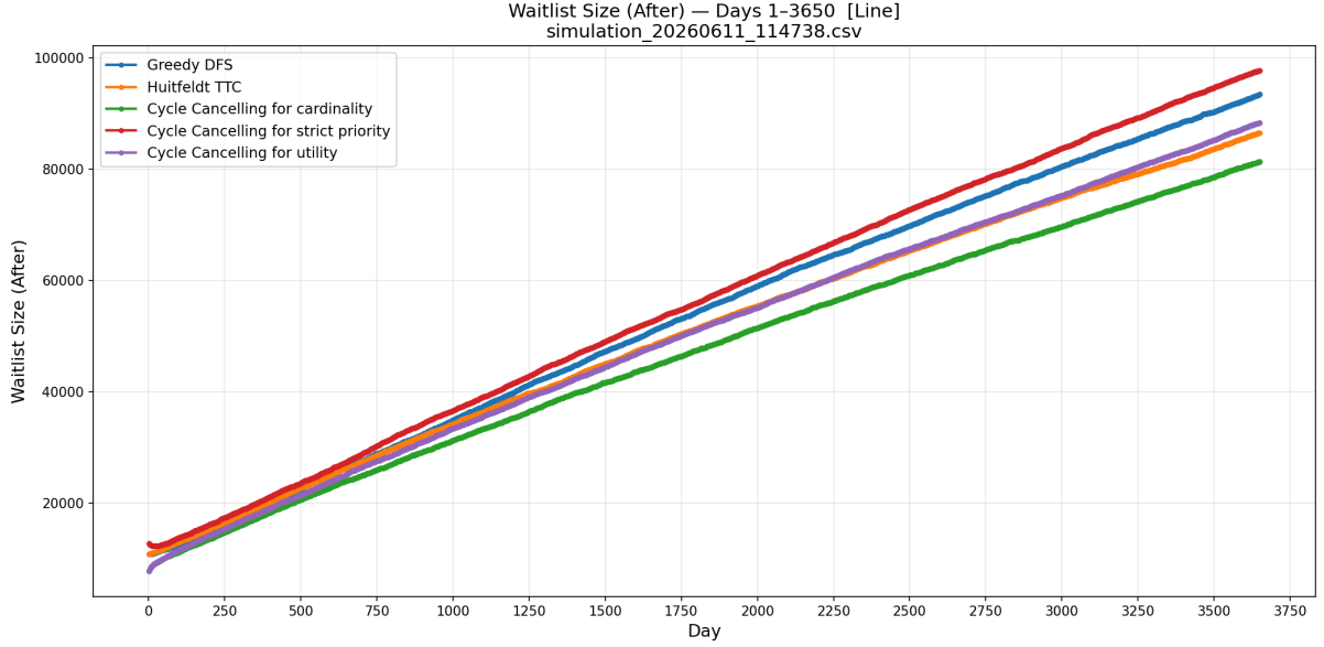
Figure 8: Waitlist size over time under each algorithm in the main simulation, over 3650 days at full scale.
