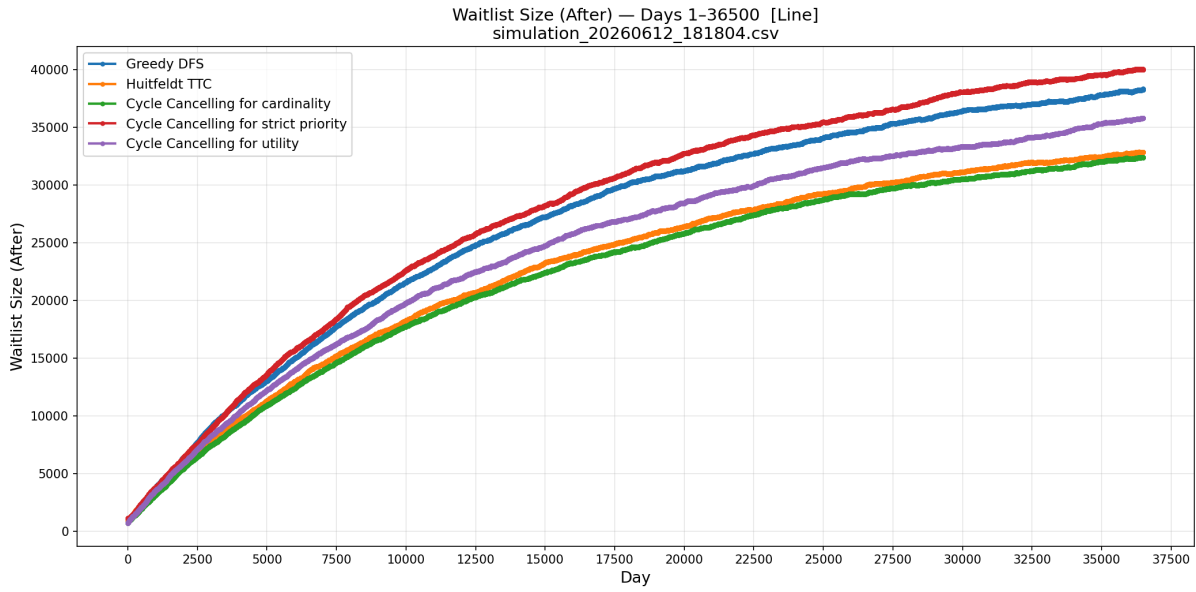
Figure 10: Waitlist size over time under each algorithm in the smaller simulation, over 100 years at one tenth scale.
