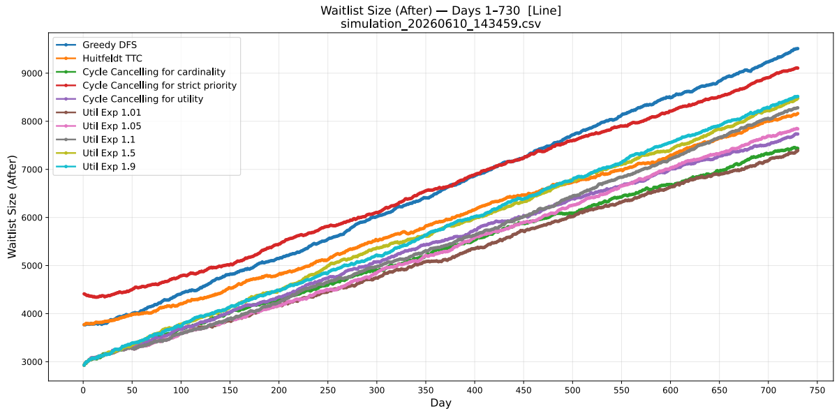
Figure 9: Waitlist size over time under each algorithm in the smaller simulation with exponential variants, over 730 days at one tenth scale.
