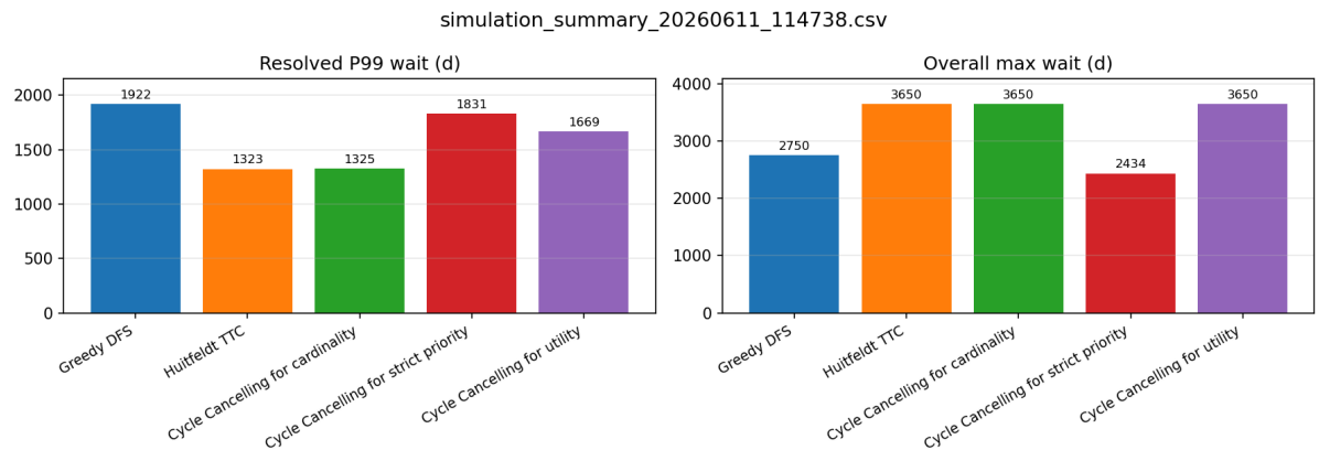
Figure 11: 99th percentile wait of resolved patients and overall maximum wait under each algorithm in the main simulation, over 3650 days. The maximum is taken over all patients, including those still waiting when the simulation ended.
