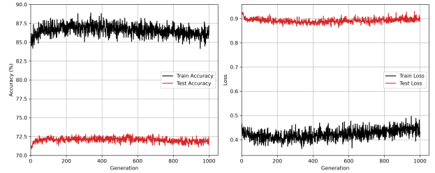
Fig. 3: Accuracy and loss during additional GA search.
