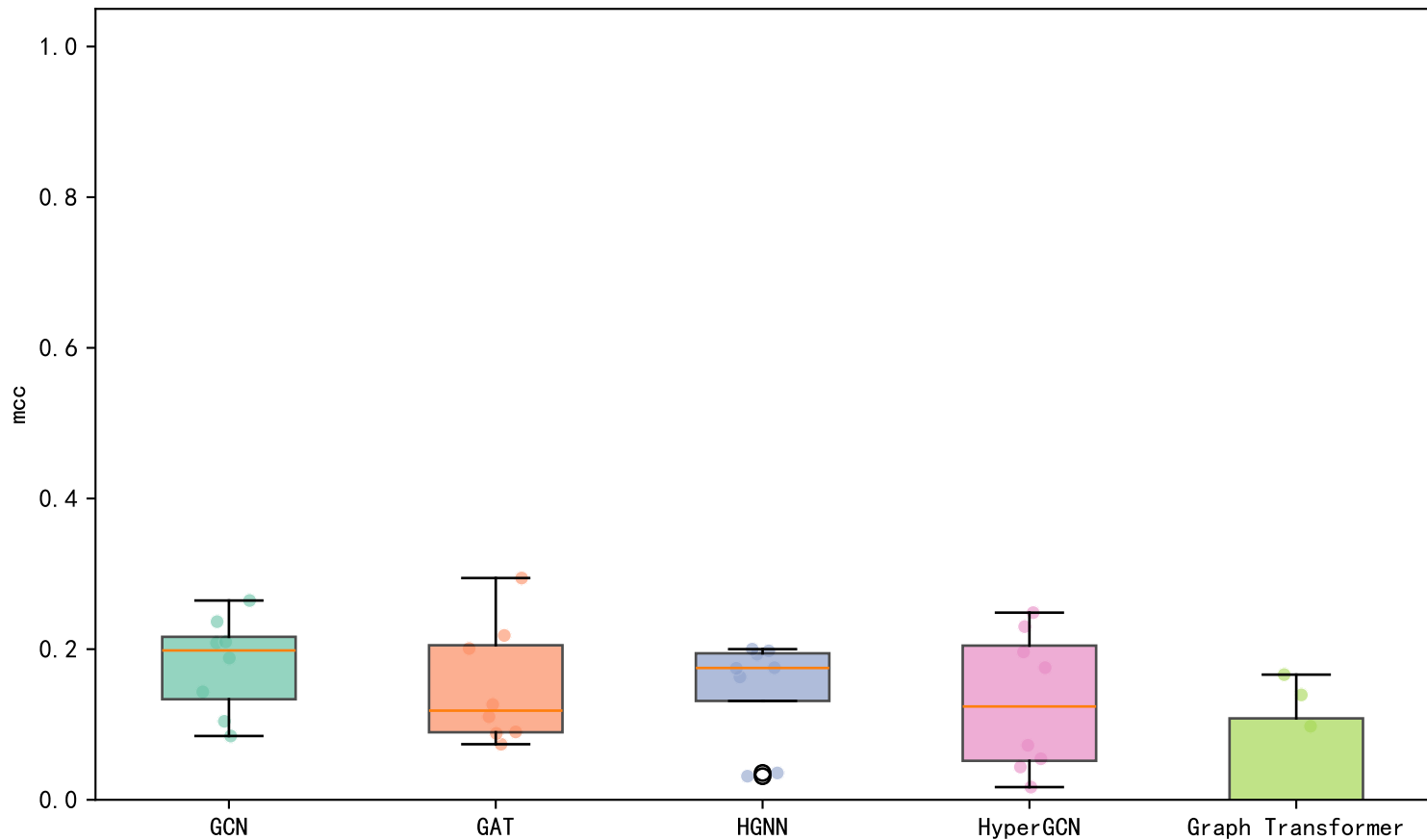
Performance Distribution — mcc
