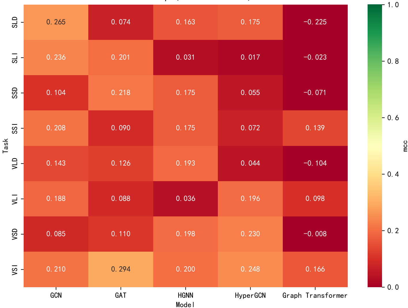
mcc Heatmap (Tasks × Models)
