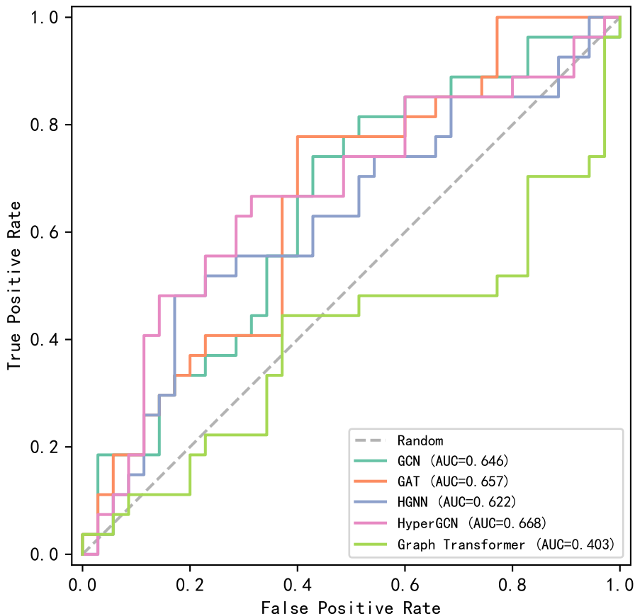
ROC Curves — SLD
