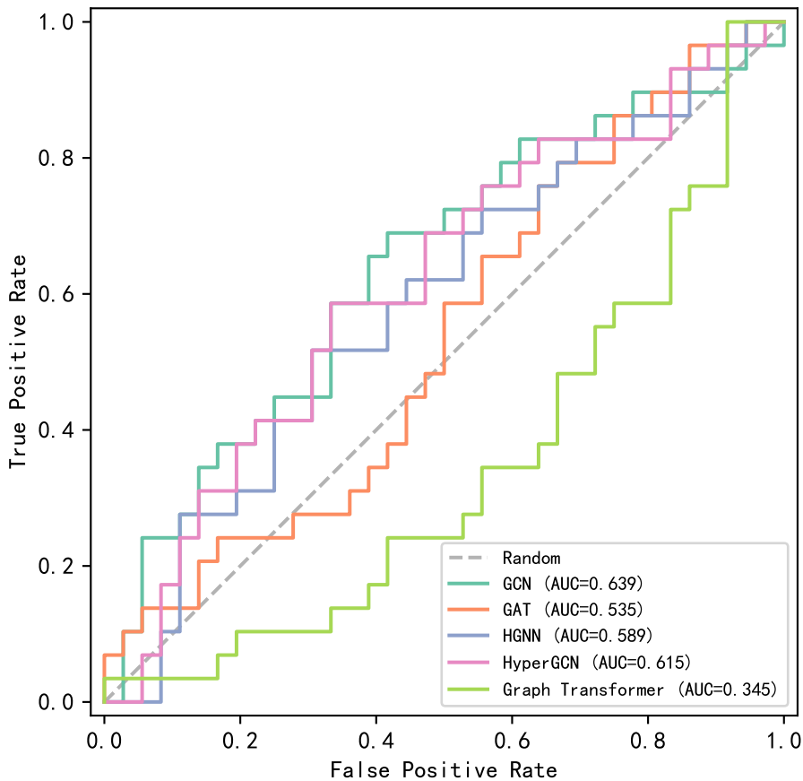
ROC Curves — SSI
