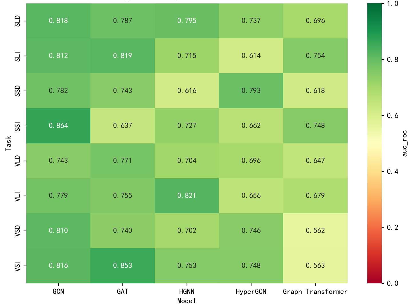
auc_roc Heatmap (Tasks × Models)
