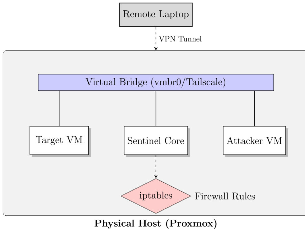
Figure 3: Network Architecture
