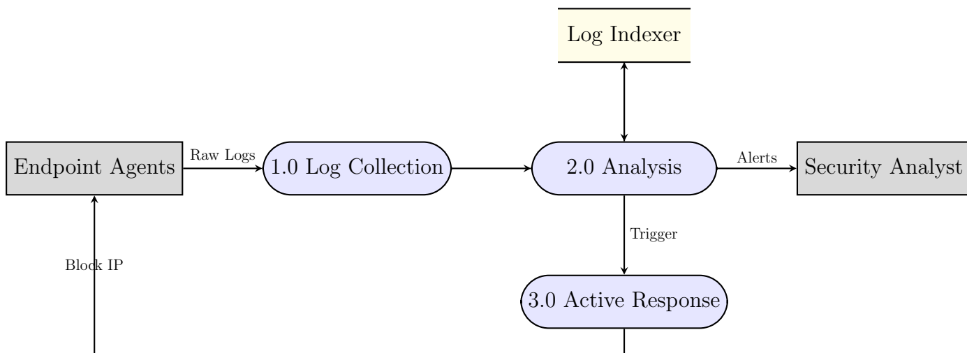
Figure 2: DFD Level 1
