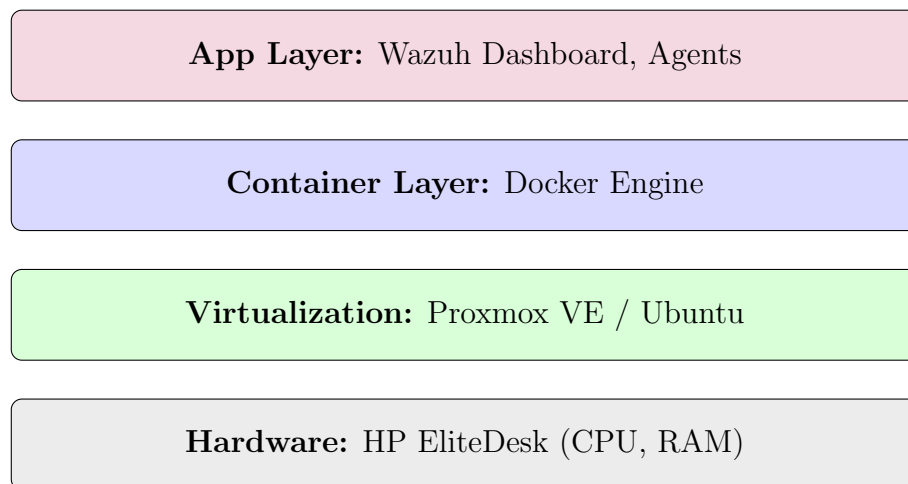
Figure 4: Technology Stack
