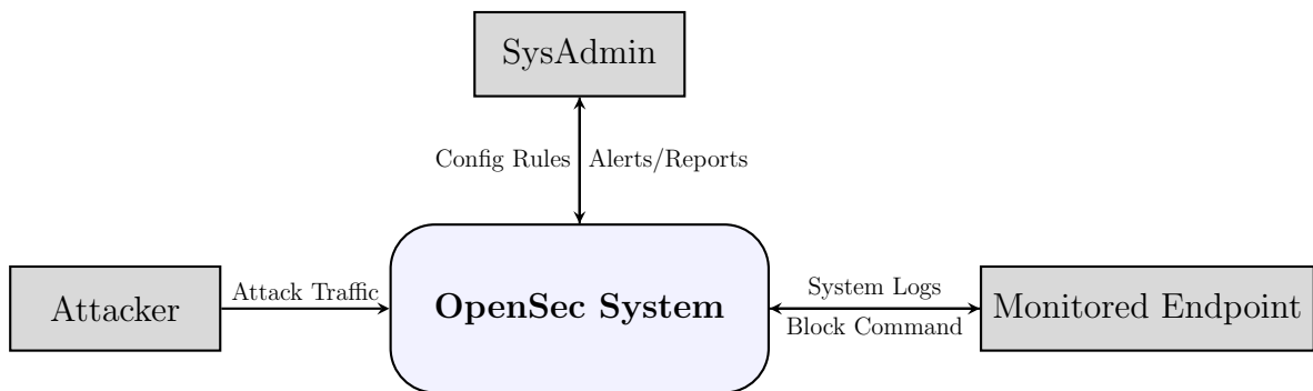
Figure 1: DFD Level 0: Context Diagram
