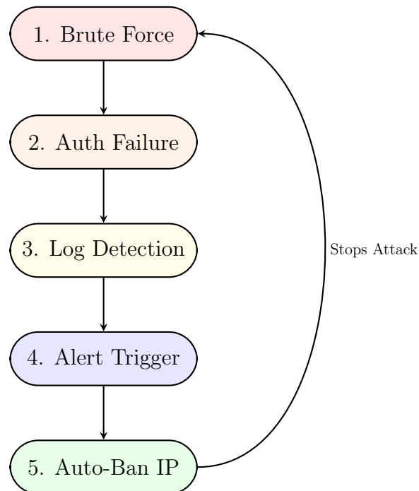
Figure 5: Incident Response Workflow
