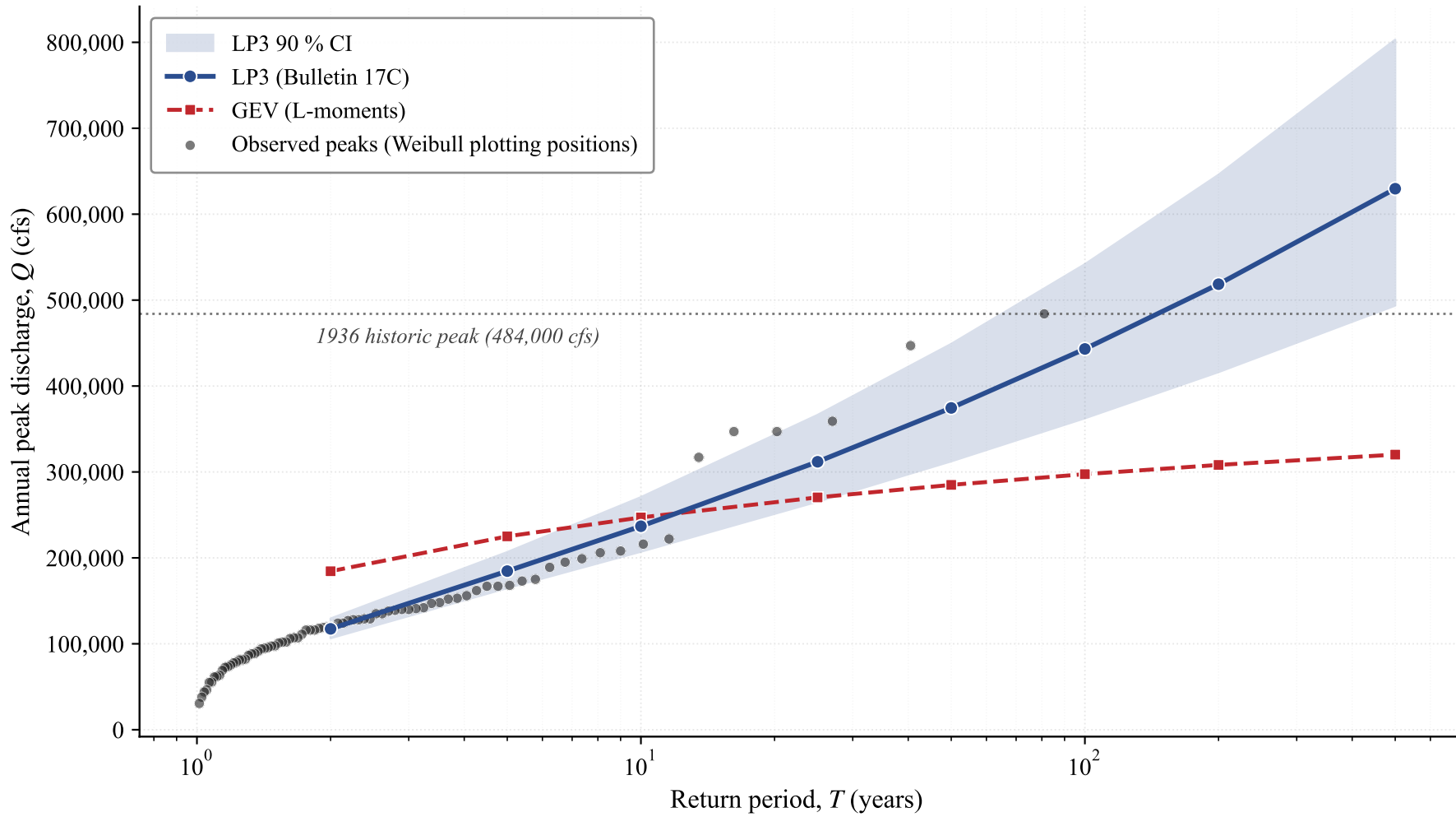
Bulletin 17C LP3 fit; GEV via L-moments shown for comparison. Shaded band: LP3 90 % confidence interval.
