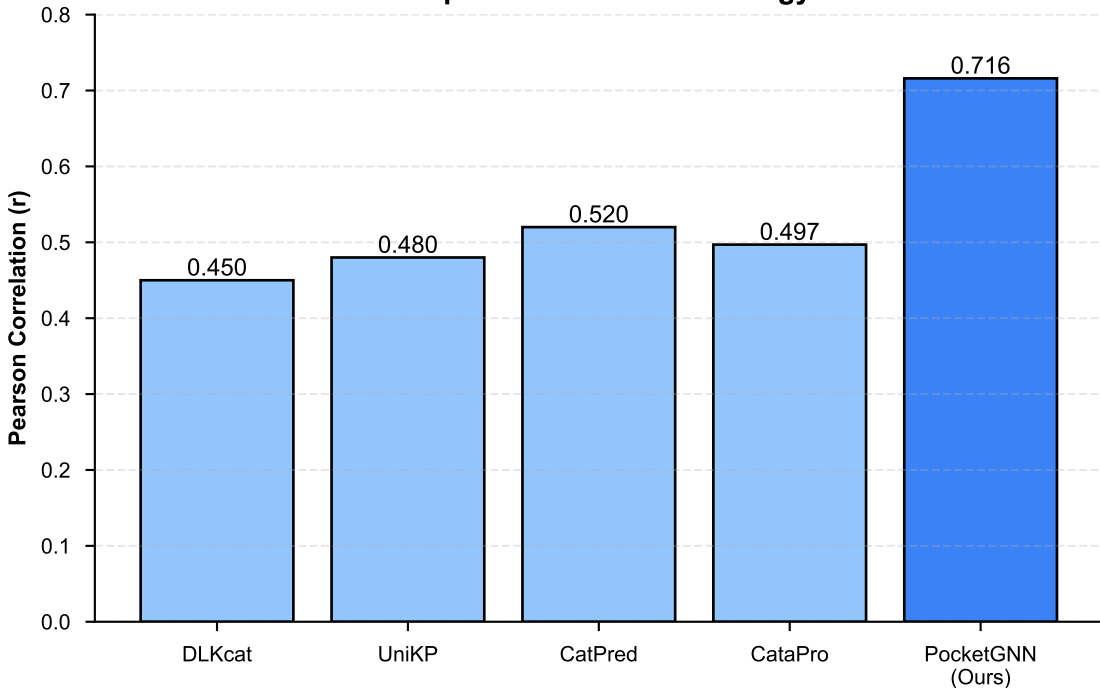
Performance Comparison on 40% Homology OOD Test Set
