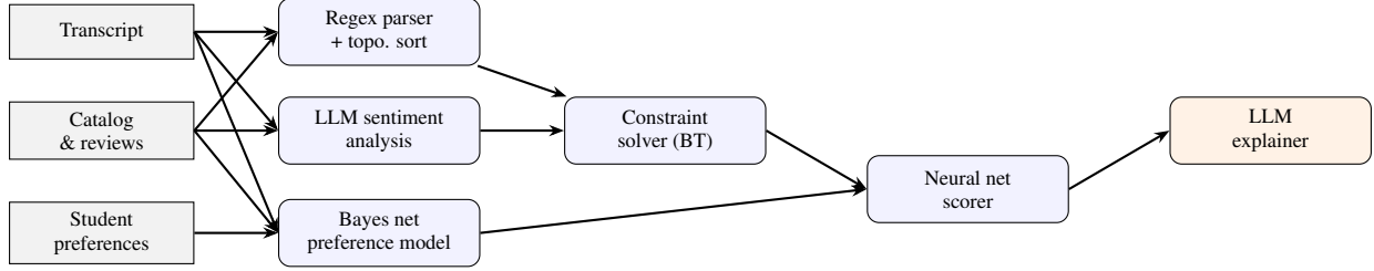
Figure 1: End-to-end pipeline. Gray nodes are data sources; blue nodes are deterministic / model components; the orange node is the LLM explainer that closes the loop with the user.
