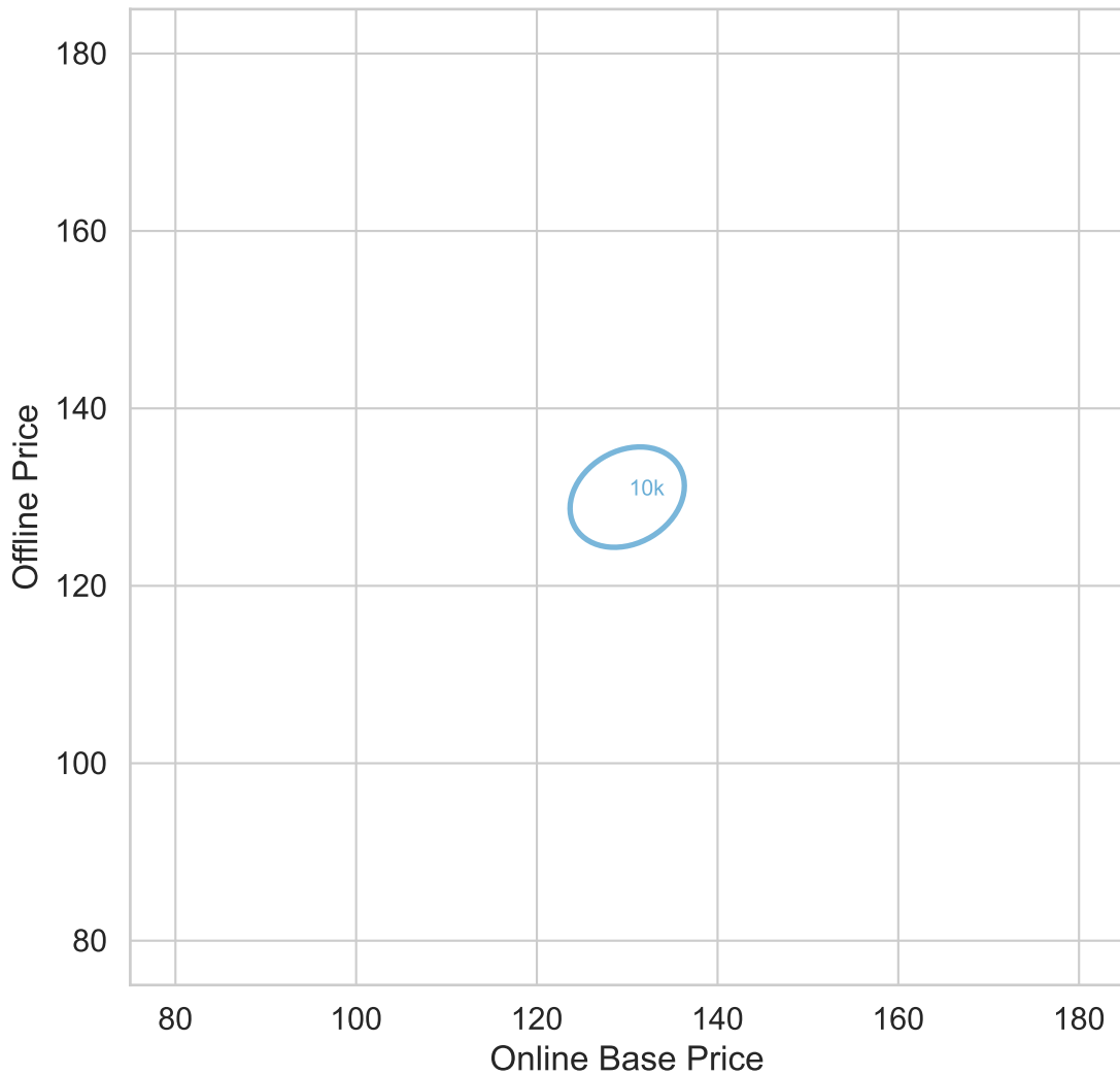
Evolution of Covariance Ellipses
