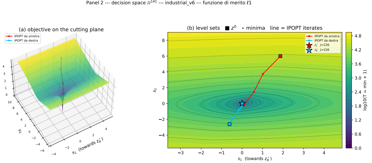
Figure 9: The objective in the decision space \mathbb{R}^{141} , on a plane constructed to contain both local minima of the recorded cycle. (a) the surface; (b) its level sets with the two minima ( \star ), the initial iterate ( \blacksquare ) and the IPOPT iterates joining them. What is plotted is not the objective f but the \ell^1 merit function T_1(z) = f(z) + \sigma \|c(z)\|_1 : in the simultaneous parametrisation X and U are independent variables tied by the dynamic equalities, so a generic point of the plane is not dynamically feasible and a plot of f alone would show a landscape the solver never traverses. The merit function is what the line search actually decreases.
