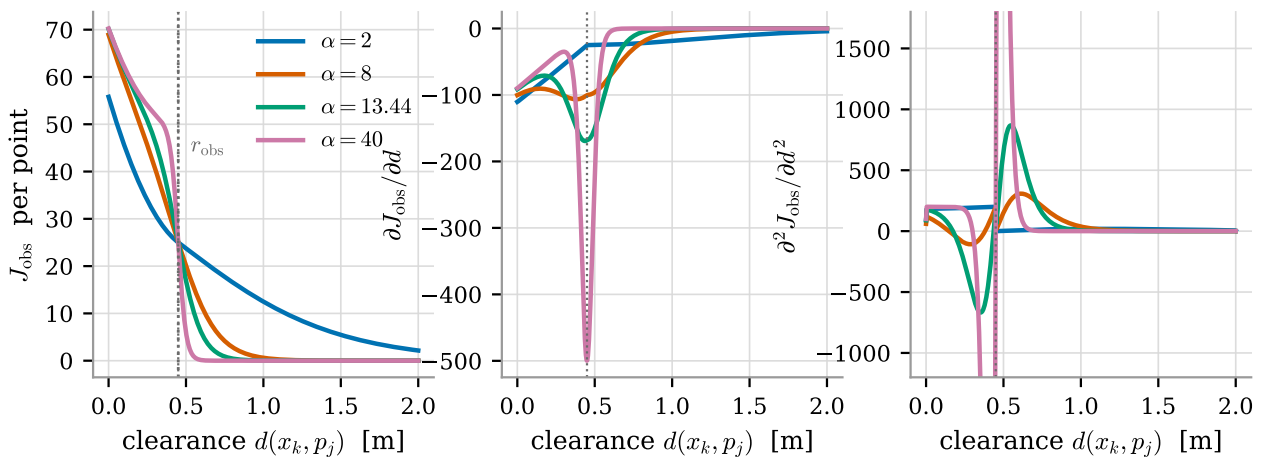
Figure 7: The hybrid barrier (24) for four steepness values ( W_{\text{obs}} = 50 , r_{\text{obs}} = 0.45 m): value (left), gradient (centre) and curvature (right) versus clearance. The sigmoid alone saturates and loses its gradient inside the obstacle; the quadratic term restores an unbounded, linearly growing restoring force for d < r_{\text{obs}} . The curvature grows as \alpha_{\text{obs}}^2 , which is what degrades the conditioning of the NLP.
