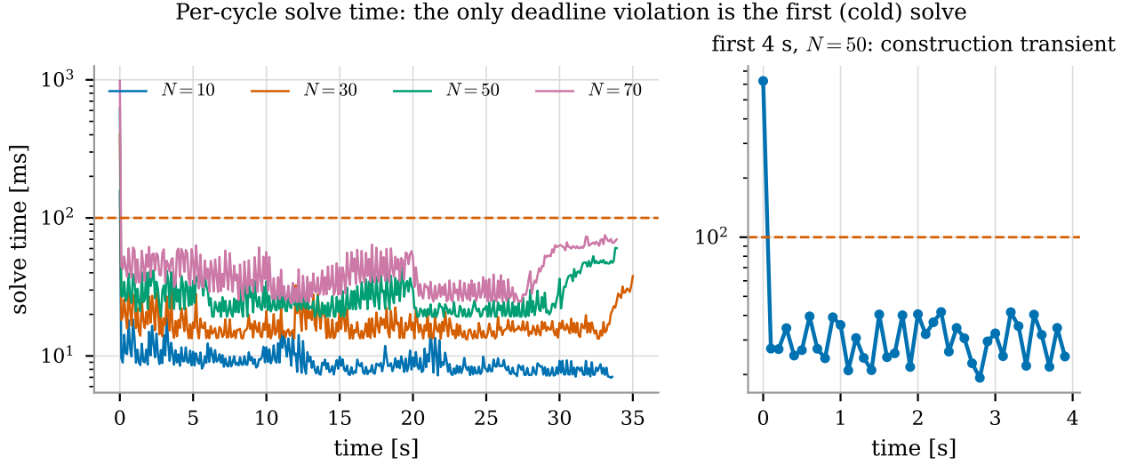
Figure 17: Per-cycle solve time (log scale) for four horizons over a full run, and a zoom on the first 4 s at N = 50 . The only deadline violation is the cold first solve, which pays the one-off NLP construction.
