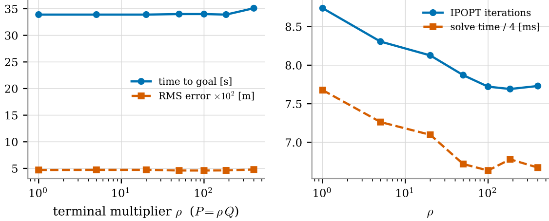
Figure 23: Terminal multiplier \rho : closed-loop performance is flat over three decades (left) while the conditioning improves slightly (right).
