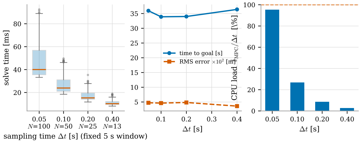
Figure 19: Sampling time at fixed look-ahead: solve-time distribution (left), closed-loop performance (centre) and duty cycle \bar{t}/\Delta t against the real-time limit (right).
