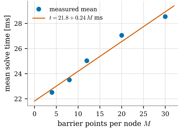
Figure 22: Mean solve time against the number of barrier points per node, with the linear fit (38). The trajectory and the iteration count are identical for all M .
