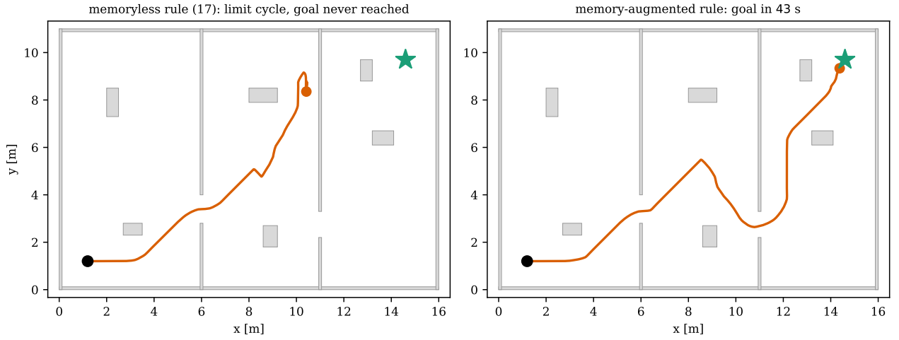
Figure 11: The rebuilt E_a under the deployed weights \theta_{\text{dep}} . Left: the memoryless rule (17) locks into a period-10 s limit cycle at the second partition and never reaches the goal. Right: the memory-augmented rule (37) turns down to the remembered doorway before ever reaching the wall and takes the goal in 43 s. Same worlds, same NLP, same weights — only the target rule differs.
