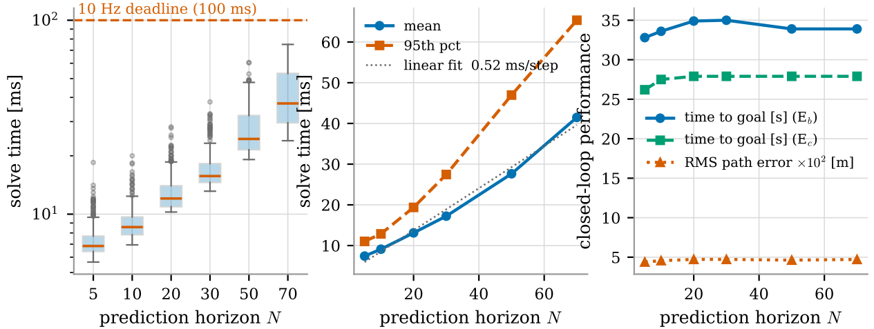
Figure 16: Prediction horizon. Left: distribution of per-cycle solve time (log scale) against the 100 ms deadline. Centre: mean and 95th percentile with a linear fit of 0.52 ms per horizon step. Right: closed-loop performance — time to goal in both worlds and RMS path error — which saturates by N \approx 20 .
