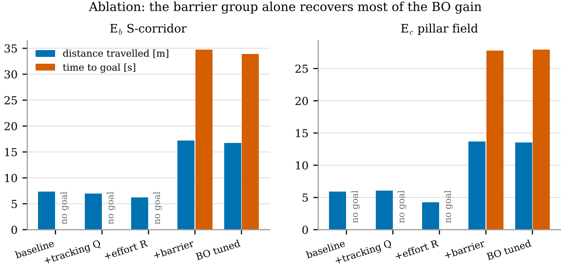
Figure 15: Ablation of the three weight groups in E_b and E_c . Only the barrier group converts a failing controller into a successful one; the effort group then recovers smoothness.
