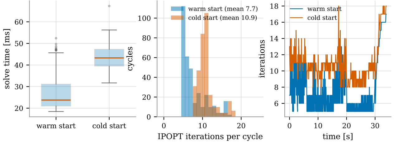
Figure 18: Warm start: solve-time distribution (left), IPOPT iteration histogram (centre) and iteration count over time (right). The executed trajectory is identical to within 10^{-4} m; only the computation changes.
