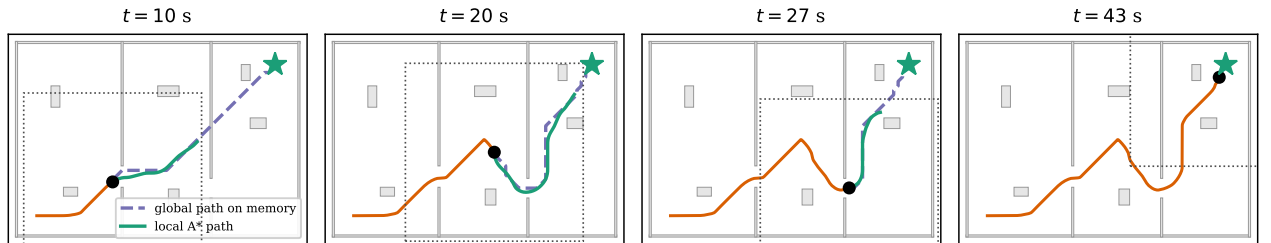
Figure 12: Four cycles of the memory-augmented rule in E_a (orange: executed trajectory; dashed: global path \pi_k on the remembered map; green: local A^* path inside the dotted 10 \times 10 m window). At t = 10 s, crossing the first doorway, the second partition is not yet in memory and \pi_k is still the optimistic near-ray; by t = 20 s the wall has been confirmed at a distance and the global path has flipped, once, to the doorway below — the robot angles down before ever reaching the wall, threads the doorway at t = 27 s and takes the goal at t = 43 s without a single reversal.
