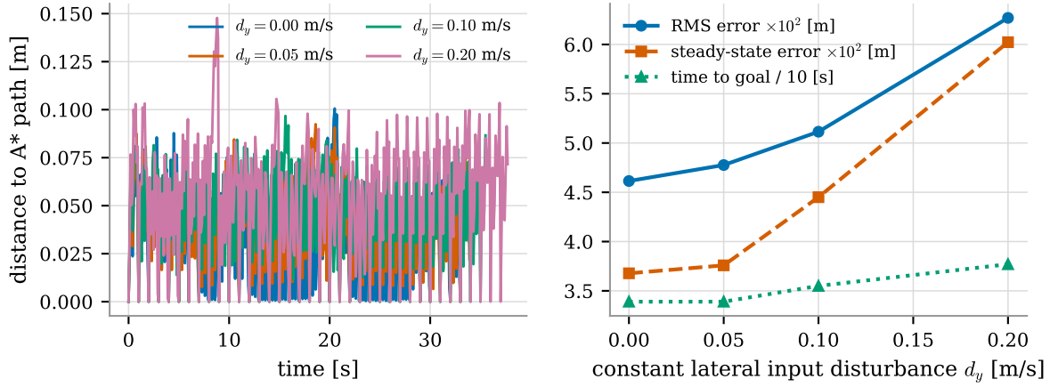
Figure 24: Model mismatch and input disturbance. Left: distance to the A^* path over time for four disturbance levels. Right: RMS error, steady-state offset and time to goal against d_y . The offset is bounded but does not vanish — the signature of a controller without integral action.
