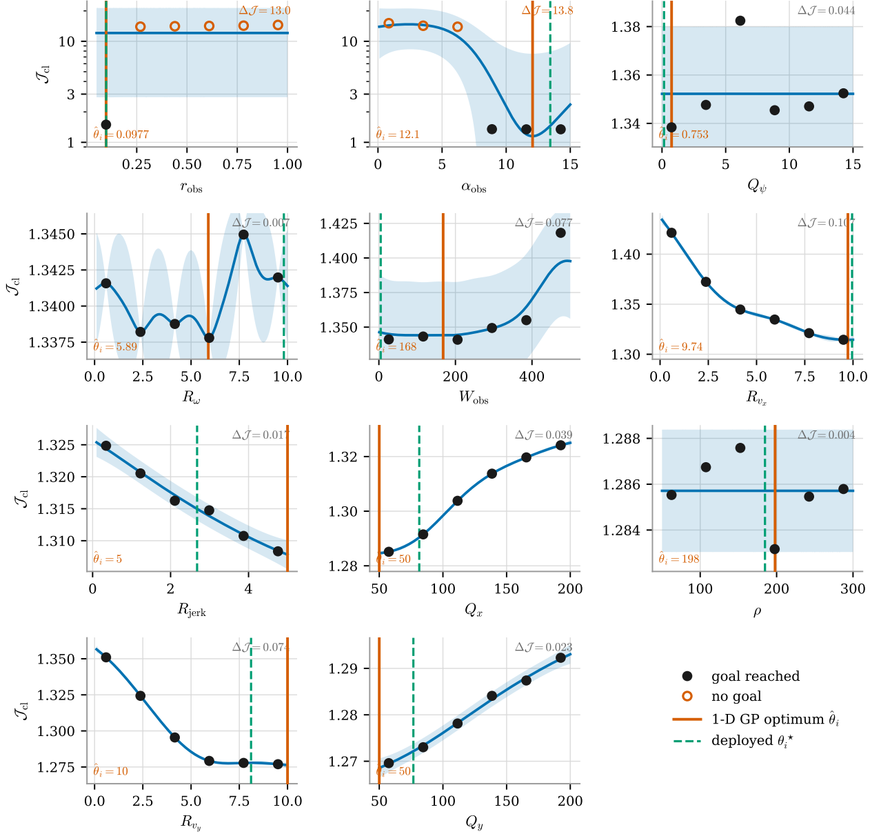
Figure 13: Closed-loop score against each single parameter: six real evaluations per axis with a 1-D GP fitted to each (band: 95% credible interval). Solid vertical line: the GP optimum \hat{\theta}_i ; dashed: the value shipped in the deployed configuration. \Delta\mathcal{J} is the spread of the six observations on that axis; panels containing a failure use a logarithmic axis, the others are zoomed to their own range. Axes are swept in the order shown, each optimum being fixed before the next axis is visited.
