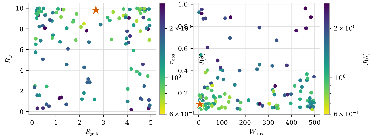
Sampling density of the 120 trials (star: incumbent \theta^* )
