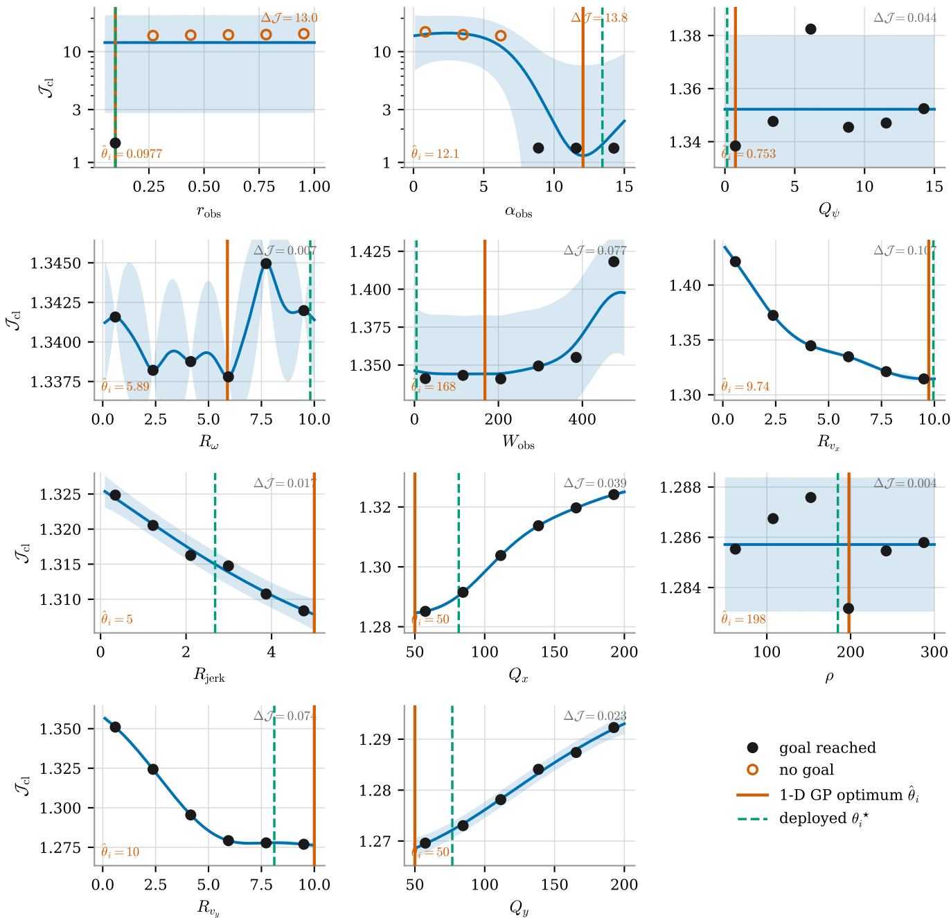
Closed-loop score against each single parameter: six real closed-loop evaluations per axis, one 1-D GP per axis ( \Delta\mathcal{J} = total spread of the six observations; panels with a failure use a log axis, the others are zoomed)
