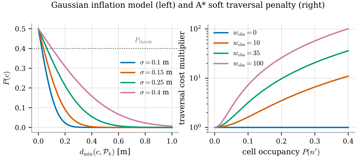
Figure 2: Left: the Gaussian inflation model (1) for four values of \sigma , with the hard threshold P_{\text{thr}} = 0.4 . Right: the soft traversal-cost multiplier 1 + w_{\text{obs}}(P/P_{\text{thr}})^2 of the A^* edge cost (6), which is what actually keeps the path away from walls; the deployed value is w_{\text{obs}} = 35 .
