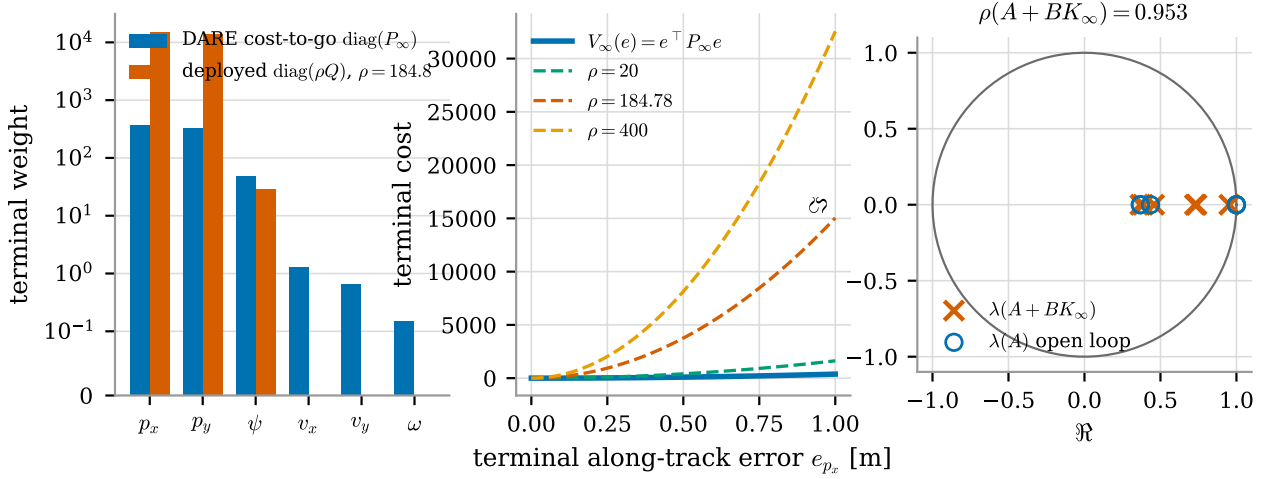
Figure 6: Terminal cost versus the infinite-horizon cost-to-go of the linearised cruise dynamics. Left: diagonal of P_\infty against the deployed \rho Q (symmetric-log scale). Centre: terminal cost along a pure along-track error for V_\infty and for three values of \rho . Right: open-loop eigenvalues of A and closed-loop eigenvalues of A + BK_\infty in the unit disc.
