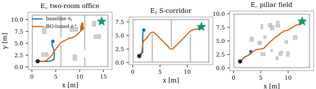
Figure 7: Executed paths in the three worlds for the baseline (blue) and the deployed weights (orange); black dot is the start, green star the goal, filled circles the final pose. The baseline stalls a few metres from the start in all three worlds; the tuned controller reaches the goal in E_b and E_c and wanders in E_a (Section 5.3).
