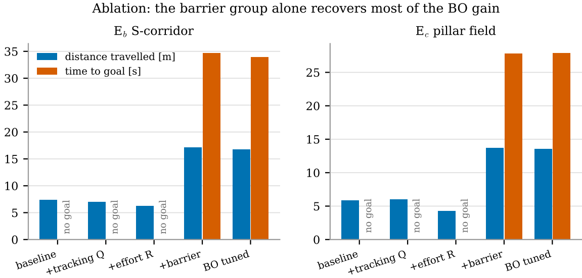
Figure 11: Ablation of the three weight groups in E_b and E_c . Only the barrier group converts a failing controller into a successful one; the effort group then recovers smoothness.
