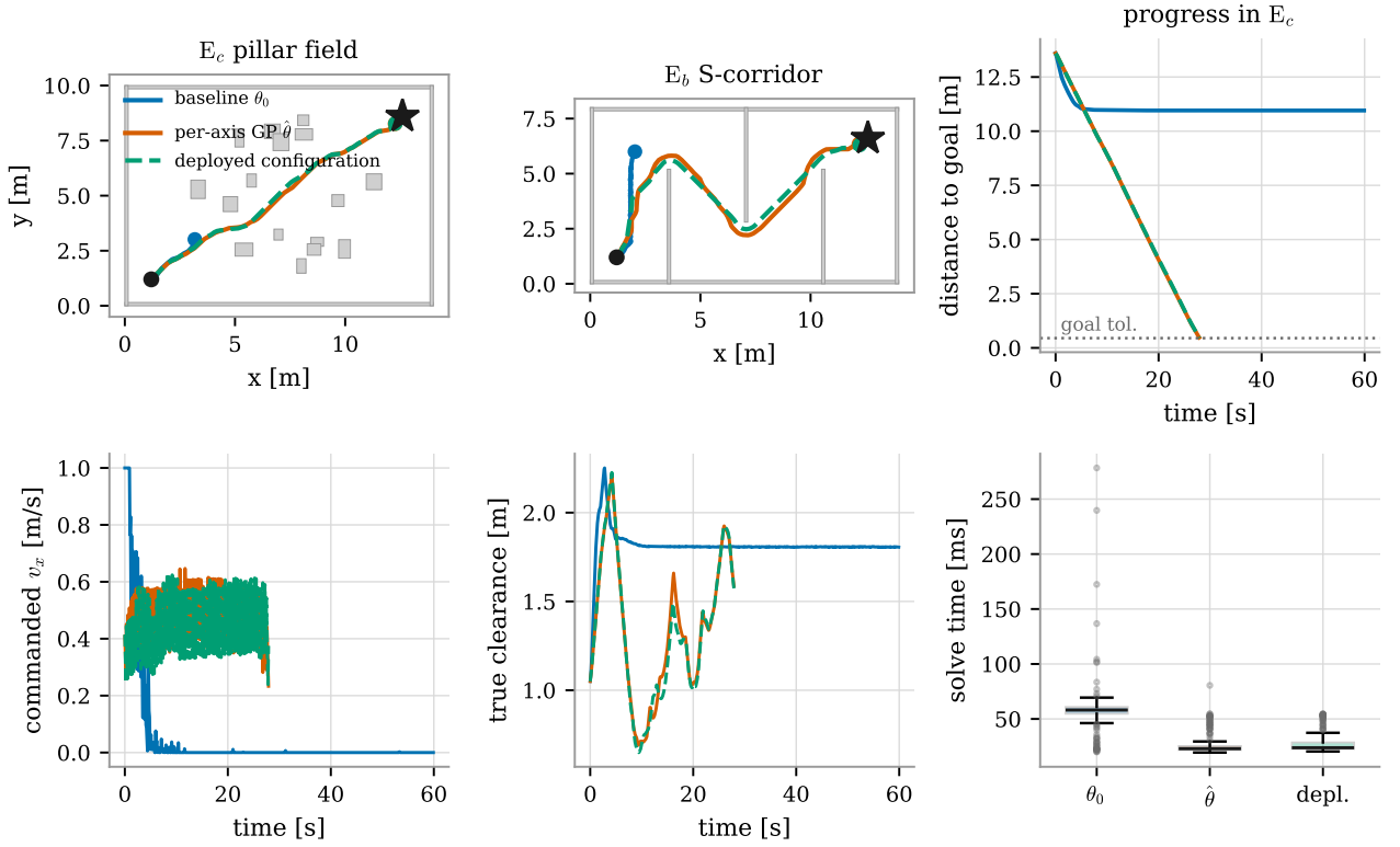
Figure 10: Executed trajectories under the baseline weights and under the weights found by the per-axis GP scheme; the deployed configuration is shown dashed for reference. Top: paths in both worlds and distance to goal against time in E_c . Bottom: commanded forward velocity, true clearance, and the distribution of per-cycle solve times.
