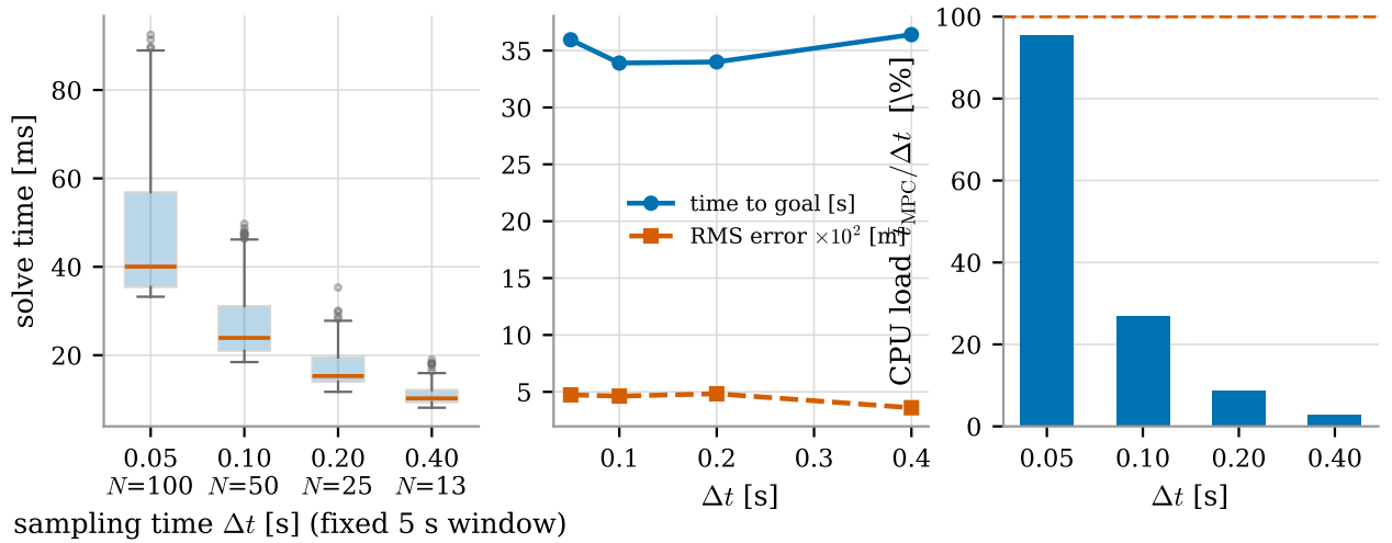
Figure 15: Sampling time at fixed look-ahead: solve-time distribution (left), closed-loop performance (centre) and duty cycle \bar{t}/\Delta t against the real-time limit (right).
