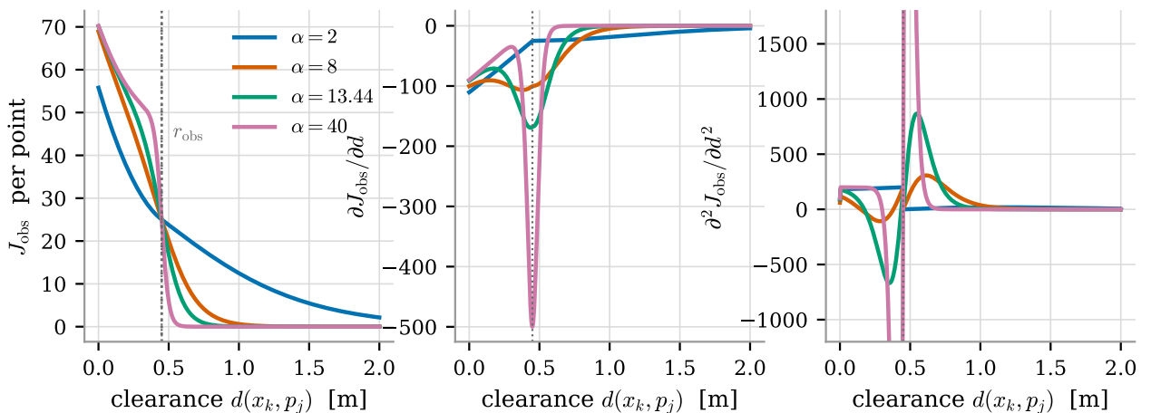
Figure 5: The hybrid barrier (15) for four steepness values ( W_{\text{obs}} = 50 , r_{\text{obs}} = 0.45 m): value (left), gradient (centre) and curvature (right) versus clearance. The sigmoid alone saturates and loses its gradient inside the obstacle; the quadratic term restores an unbounded, linearly growing restoring force for d < r_{\text{obs}} . The curvature grows as \alpha_{\text{obs}}^2 , which is what degrades the conditioning of the NLP.
