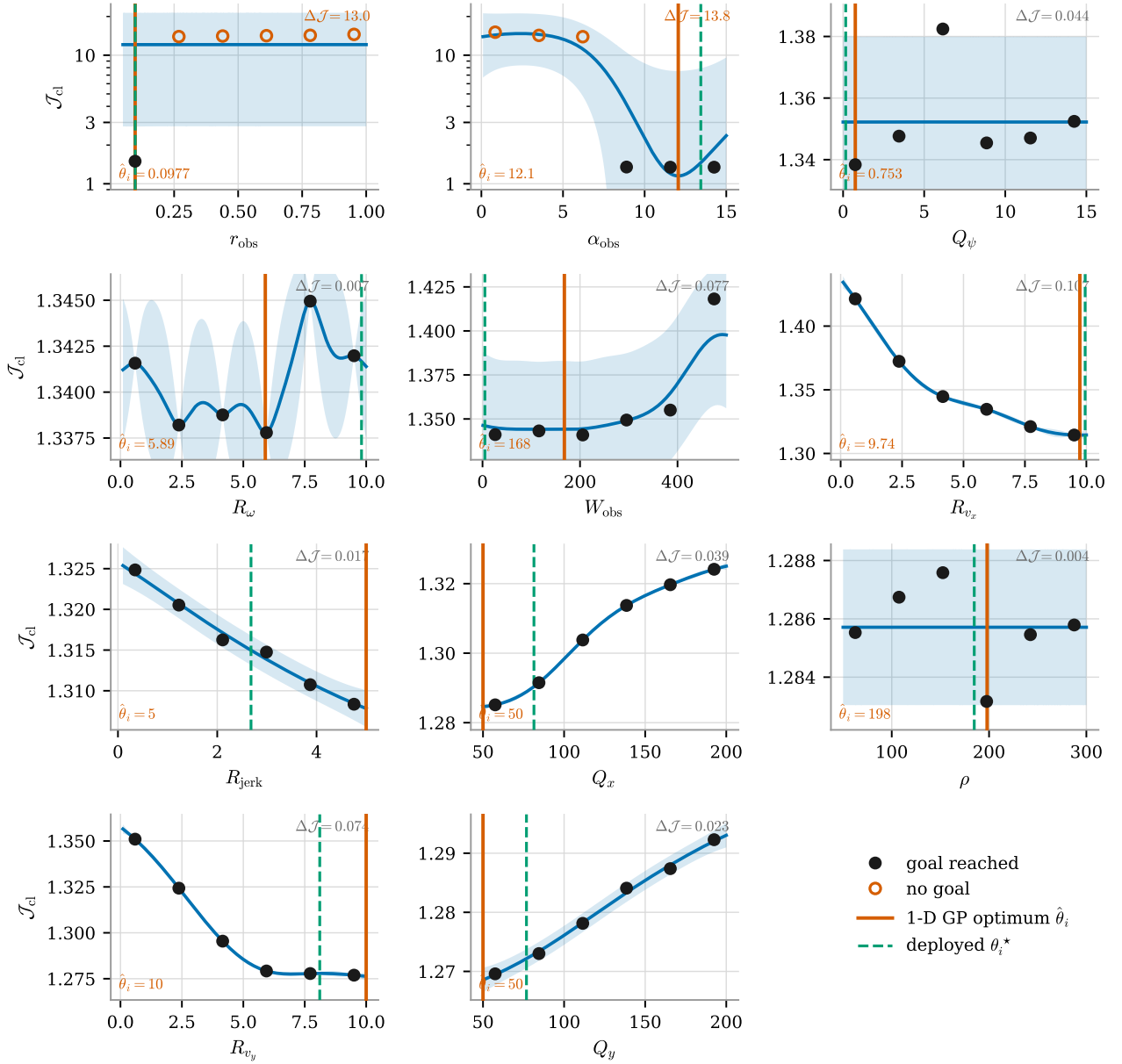
Figure 9: Closed-loop score against each single parameter: six real evaluations per axis with a 1-D GP fitted to each (band: 95% credible interval). Solid vertical line: the GP optimum \hat{\theta}_i ; dashed: the value shipped in the deployed configuration. \Delta\mathcal{J} is the spread of the six observations on that axis; panels containing a failure use a logarithmic axis, the others are zoomed to their own range. Axes are swept in the order shown, each optimum being fixed before the next axis is visited.
