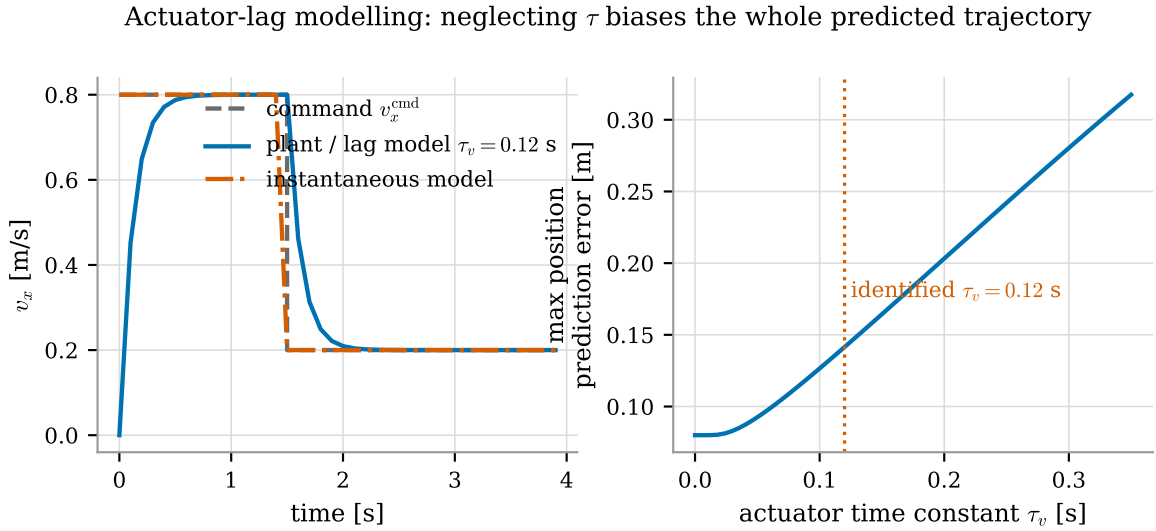
Figure 3: Actuator-lag modelling. Left: response of the first-order-lag model (3) against the instantaneous model v \equiv u for a step in commanded forward velocity. Right: maximum position prediction error accumulated over one 5 s horizon by neglecting the lag, as a function of \tau_v .
