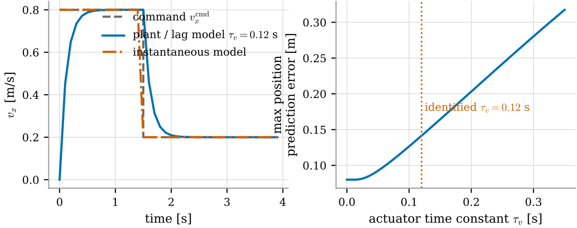
Figure 5: Actuator-lag modelling. Left: response of the first-order-lag model (11) against the instantaneous model v \equiv u for a step in commanded forward velocity. Right: maximum position prediction error accumulated over one 5 s horizon by neglecting the lag, as a function of \tau_v .
