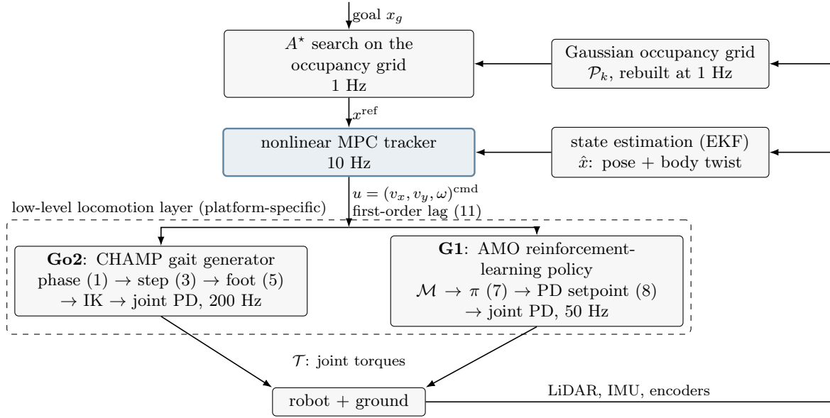
Figure 3: Cascaded structure of the controller, from the goal down to joint torques. The report analyses the two stages at the top; everything inside the dashed box is a platform-specific locomotion layer that the MPC sees only through the first-order lag (11), which is the abstraction seam of the design. The rates fall by roughly a decade at every seam (1 Hz, 10 Hz, 50–200 Hz, motor-driver rate), which is what allows the layers to be designed separately, and the two branches inside the dashed box — a hand-designed gait generator and a learned policy — are interchangeable precisely because they present the same twist interface u .
