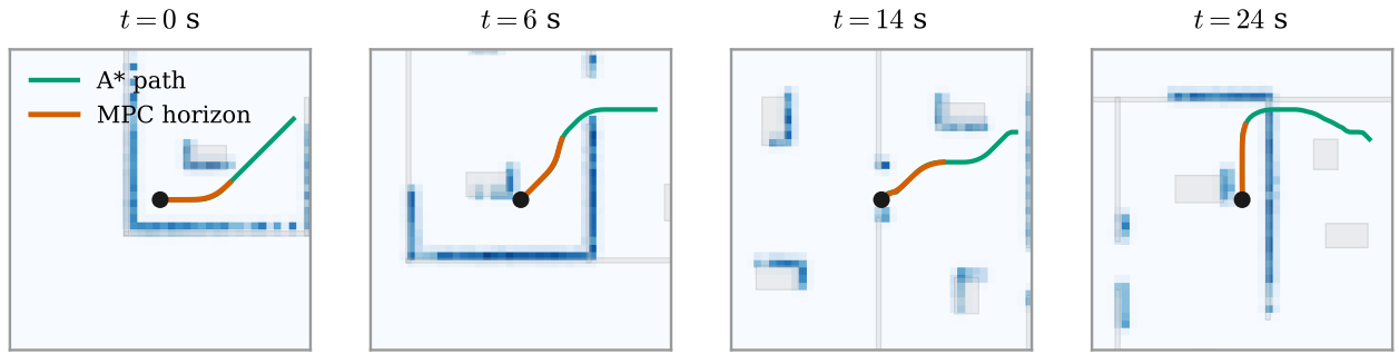
Figure 10: Four snapshots of a rolling-horizon cycle in E_a (blue field: Gaussian occupancy in the moving 10 \times 10 m window; green: A^* path; orange: MPC prediction). The optimization is solved correctly at every cycle — the failure is in the greedy target rule (16), not in the NLP.
