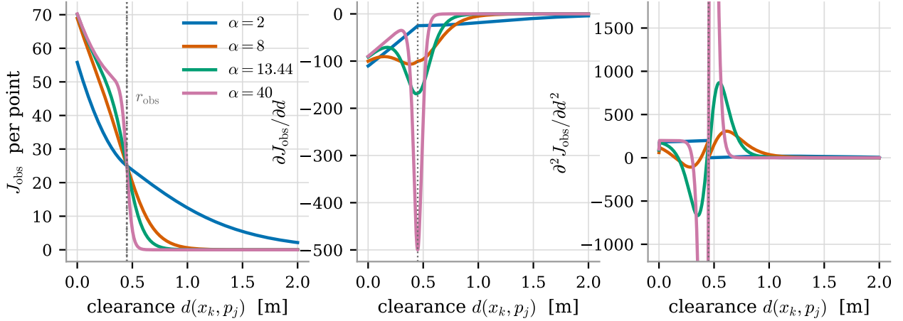
Figure 7: The hybrid barrier (23) for four steepness values ( W_{\text{obs}} = 50 , r_{\text{obs}} = 0.45 m): value (left), gradient (centre) and curvature (right) versus clearance. The sigmoid alone saturates and loses its gradient inside the obstacle; the quadratic term restores an unbounded, linearly growing restoring force for d < r_{\text{obs}} . The curvature grows as \alpha_{\text{obs}}^2 , which is what degrades the conditioning of the NLP.
