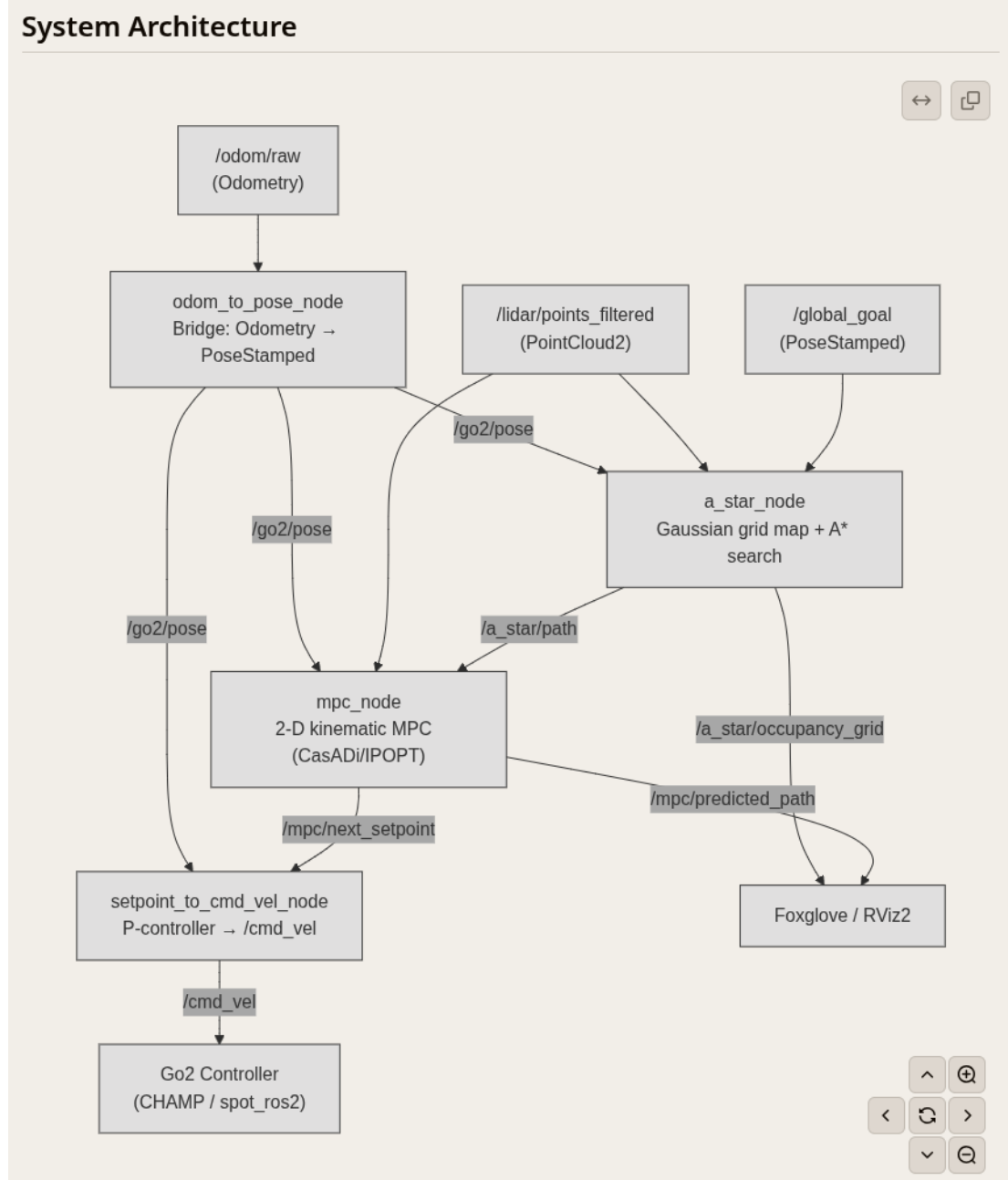
Figure 1: Architecture of the navigation stack. The two runtime optimization programs analysed in this report are the A^* search on the Gaussian occupancy grid and the nonlinear MPC tracker; the Bayesian tuning stage is executed offline and only produces the weight vector \hat{\theta} .
