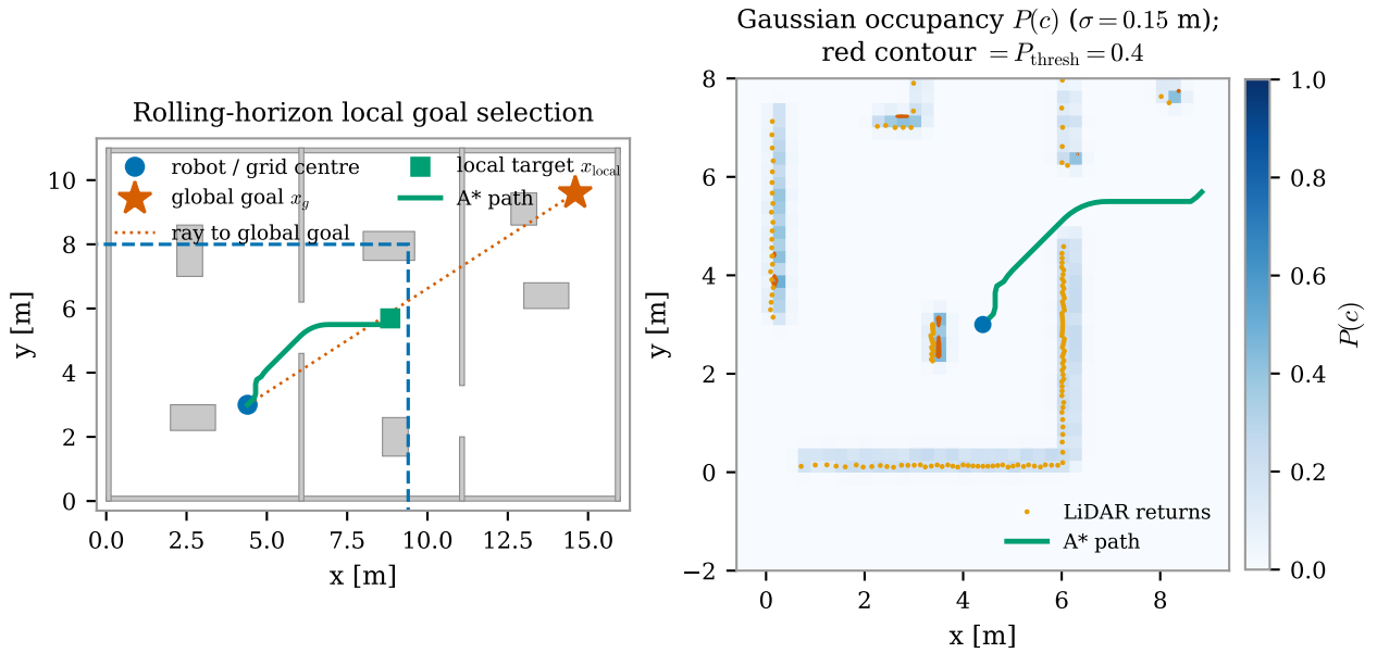
Figure 6: Left: rolling-horizon target selection (16) — the dashed square is the 10 \times 10 m local grid, the dotted line the ray to the global goal, the square marker the local target where that ray meets the grid boundary, and the solid line the A^* solution. Right: the Gaussian occupancy field (9) built from the current returns, with the P = 0.4 hard-obstacle contour.
