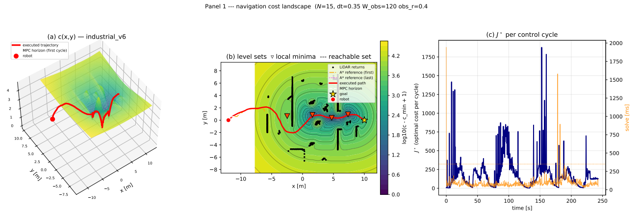
Figure 6: The navigation cost landscape of the recorded run industrial_v6 . (a) the surface c(p) of Eq. (28) over the world plane, with the executed trajectory (red) and one MPC horizon (dashed) drawn on the surface: the obstacle term raises a ridge along every wall of the plant, the tracking term forms the valley along the A^* reference. (b) the same field as level sets, with the local minima marked and the shaded region showing the set reachable within one horizon under \mathcal{U} — the constraint, not the cost, is what excludes most of the plane. (c) the optimal cost J^* of each control cycle, and the solve time beside it. The point worth noticing is in panel (a): the trajectory does not follow steepest descent , and climbs the surface wherever doing so lowers the sum over the horizon.
